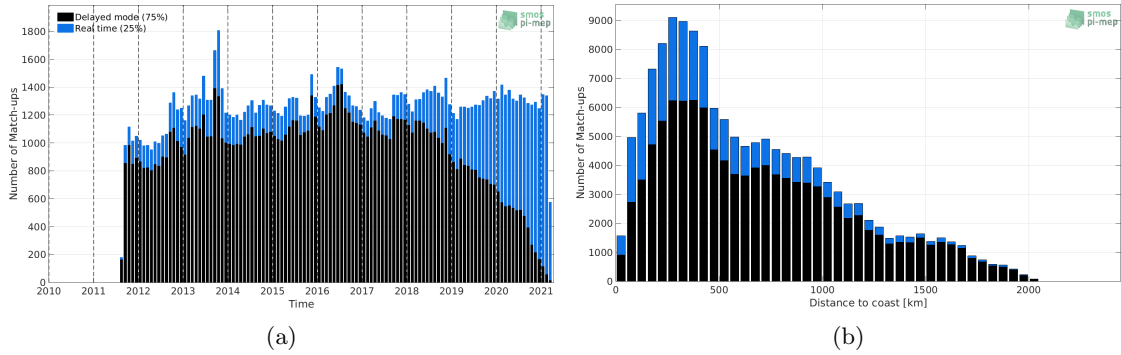
Figure 1: Number of match-ups between Argo and SMAP SSS L4 OI v1 - 7day (IPRC) SSS as a function of time (a) and as function of the distance to coast (b) over the North Atlantic Ocean Pi-MEP region and for the full satellite product period.
