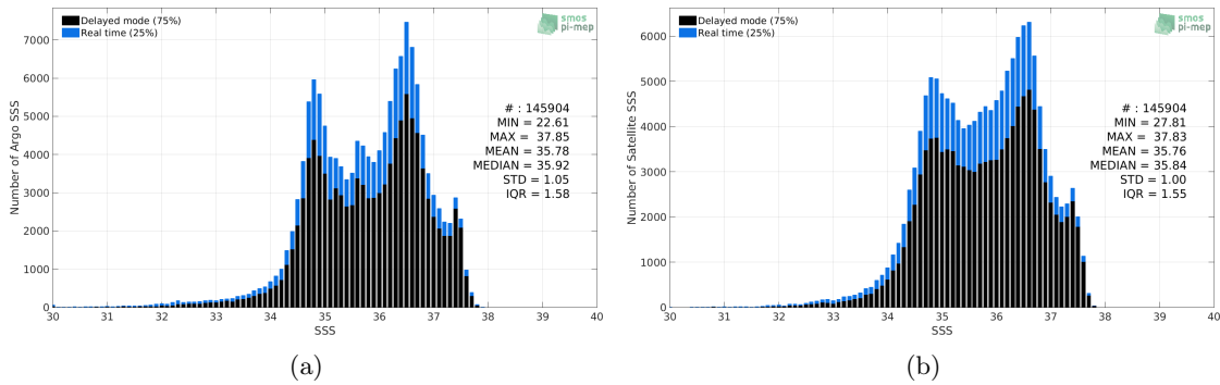
Figure 2: Histograms of SSS from Argo (a) and SMAP SSS L4 OI v1 - 7day (IPRC) (b) considering all match-up pairs per bins of 0.1 over the North Atlantic Ocean Pi-MEP region and for the full satellite product period.
