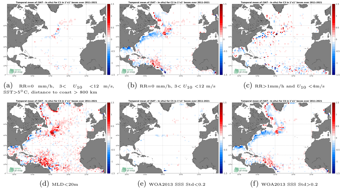
Figure 12: Temporal mean gridded over spatial boxes of size 1^\circ \times 1^\circ of \Delta SSS (SMAP SSS L4 OI v1 - 7day (IPRC) - Argo) for 6 different subdatasets corresponding to: RR=0 mm/h, 3 < U_{10} < 12 m/s, SST > 5^\circ C , distance to coast > 800 km (a), RR=0 mm/h, 3 < U_{10} < 12 m/s (b), RR > 1 mm/h and U_{10} < 4 m/s (c), MLD < 20 m (d), WOA2013 SSS Std < 0.2 (e), WOA2013 SSS Std > 0.2 (f).
