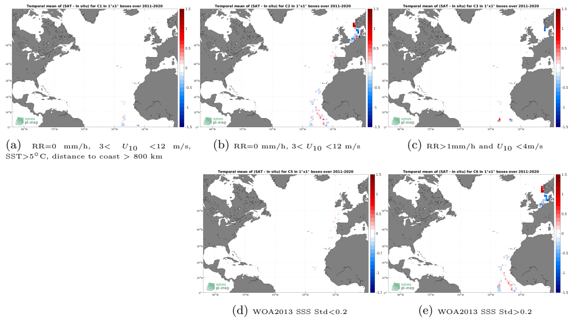
Figure 12: Temporal mean gridded over spatial boxes of size 1^\circ \times 1^\circ of \Delta SSS (SMAP SSS L4 OI v1 - Monthly (IPRC) - TSG (Polarstern)) for 5 different subdatasets corresponding to:RR=0 mm/h, 3 < U_{10} < 12 m/s, SST > 5^\circ\text{C} , distance to coast > 800 km (a), RR=0 mm/h, 3 < U_{10} < 12 m/s (b), RR > 1 mm/h and U_{10} < 4 m/s (c), WOA2013 SSS Std < 0.2 (d), WOA2013 SSS Std > 0.2 (e).
