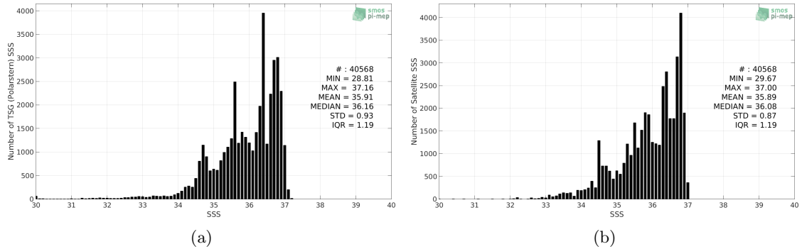
Figure 2: Histograms of SSS from TSG (Polarstern) (a) and SMAP SSS L4 OI v1 - Monthly (IPRC) (b) considering all match-up pairs per bins of 0.1 over the North Atlantic Ocean Pi-MEP region and for the full satellite product period.
