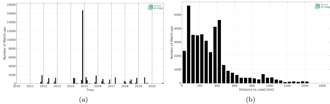
Figure 1: Number of match-ups between TSG (Polarstern) and SMAP SSS L4 OI v1 - Monthly (IPRC) SSS as a function of time (a) and as function of the distance to coast (b) over the North Atlantic Ocean Pi-MEP region and for the full satellite product period.
