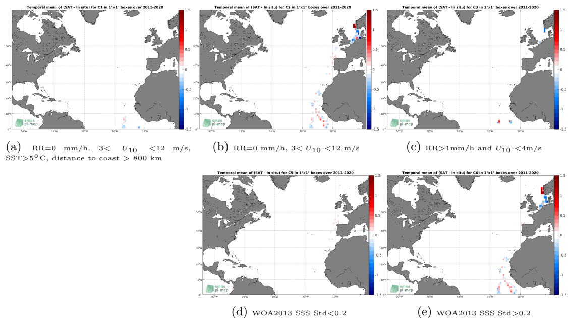
Figure 12: Temporal mean gridded over spatial boxes of size 1^\circ \times 1^\circ of \Delta SSS (SMAP SSS L4 OI v1 - Monthly (IPRC) - TSG (Polarstern)) for 5 different subdatasets corresponding to: RR=0 mm/h, 3 < U_{10} < 12 m/s, SST > 5^\circ\text{C} , distance to coast > 800 km (a), RR=0 mm/h, 3 < U_{10} < 12 m/s (b), RR > 1 mm/h and U_{10} < 4 m/s (c), WOA2013 SSS Std < 0.2 (d), WOA2013 SSS Std > 0.2 (e).
