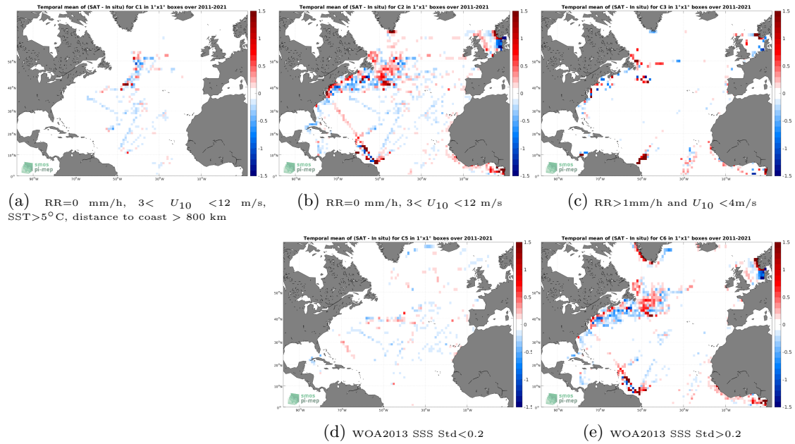
Figure 12: Temporal mean gridded over spatial boxes of size 1^\circ \times 1^\circ of \Delta\text{SSS} (SMAP SSS L4 OI v1 - Monthly (IPRC) - TSG (LEGOS-DM)) for 5 different subdatasets corresponding to:RR=0 mm/h, 3 < U_{10} < 12 m/s, SST >5^\circ\text{C} , distance to coast > 800 km (a), RR=0 mm/h, 3 < U_{10} < 12 m/s (b), RR >1 mm/h and U_{10} < 4 m/s (c), WOA2013 SSS Std <0.2 (d), WOA2013 SSS Std >0.2 (e).
