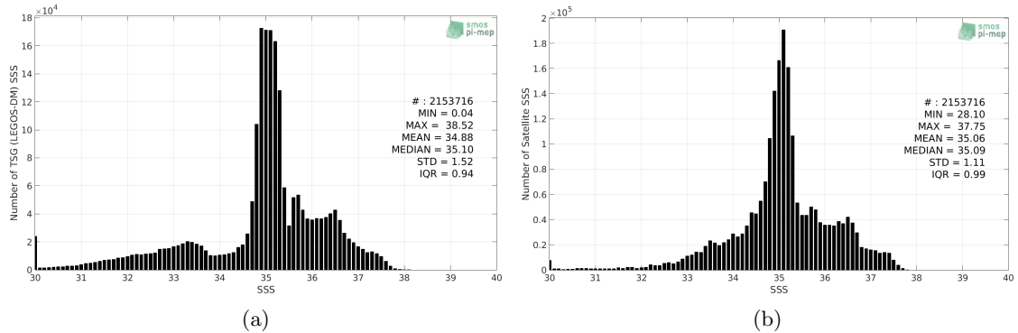
Figure 2: Histograms of SSS from TSG (LEGOS-DM) (a) and SMAP SSS L4 OI v1 - Monthly (IPRC) (b) considering all match-up pairs per bins of 0.1 over the North Atlantic Ocean Pi-MEP region and for the full satellite product period.
