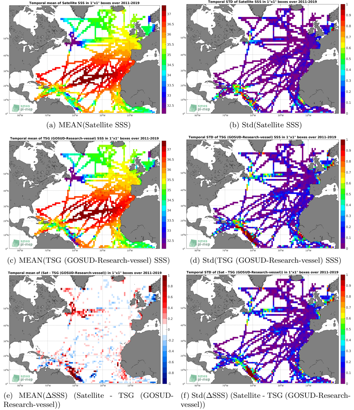
Figure 6: Temporal mean (left) and Std (right) of SSS from SMAP SSS L4 OI v1 - Monthly (IPRC) (top), TSG (GOSUD-Research-vessel) (middle), and of \Delta SSS (Satellite - TSG (GOSUD-Research-vessel)). Only match-up pairs are used to generate these maps.
