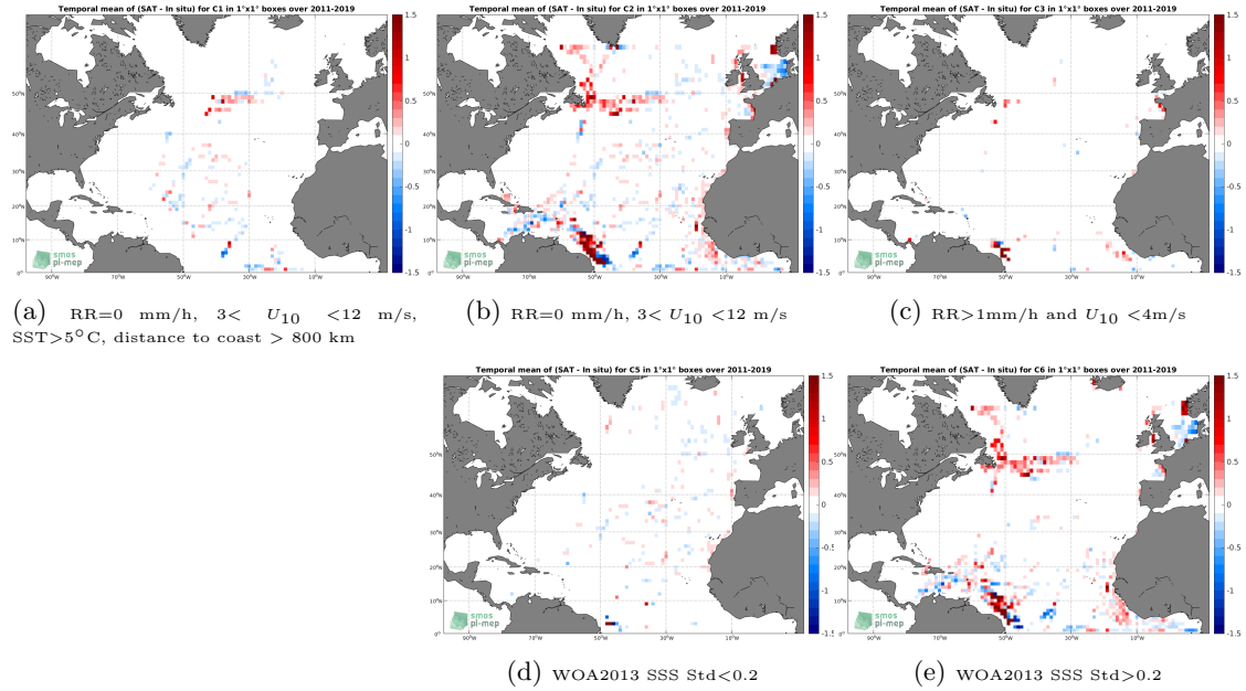
Figure 12: Temporal mean gridded over spatial boxes of size 1^\circ \times 1^\circ of \Delta SSS (SMAP SSS L4 OI v1 - Monthly (IPRC) - TSG (GOSUD-Research-vessel)) for 5 different subdatasets corresponding to: RR=0 mm/h, 3 < U_{10} < 12 m/s, SST > 5^\circ\text{C} , distance to coast > 800 km (a), RR=0 mm/h, 3 < U_{10} < 12 m/s (b), RR > 1 mm/h and U_{10} < 4 m/s (c), WOA2013 SSS Std < 0.2 (d), WOA2013 SSS Std > 0.2 (e).
