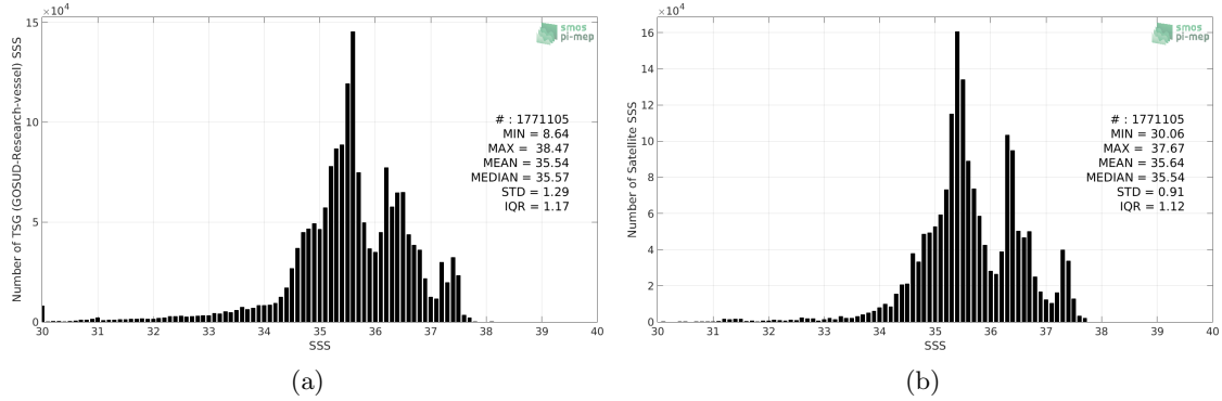
Figure 2: Histograms of SSS from TSG (GOSUD-Research-vessel) (a) and SMAP SSS L4 OI v1 - Monthly (IPRC) (b) considering all match-up pairs per bins of 0.1 over the North Atlantic Ocean Pi-MEP region and for the full satellite product period.
