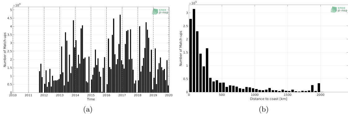
Figure 1: Number of match-ups between TSG (GOSUD-Research-vessel) and SMAP SSS L4 OI v1 - Monthly (IPRC) SSS as a function of time (a) and as function of the distance to coast (b) over the North Atlantic Ocean Pi-MEP region and for the full satellite product period.
