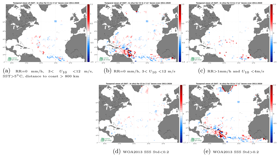
Figure 11: Temporal mean gridded over spatial boxes of size 1^\circ \times 1^\circ of \Delta\text{SSS} (SMAP SSS L4 OI v1 - Monthly (IPRC) - Surface drifters) for 5 different subdatasets corresponding to:RR=0 mm/h, 3 < U_{10} < 12 m/s, SST >5^\circ\text{C} , distance to coast > 800 km (a), RR=0 mm/h, 3 < U_{10} < 12 m/s (b), RR >1 mm/h and U_{10} < 4 m/s (c), WOA2013 SSS Std <0.2 (d), WOA2013 SSS Std >0.2 (e).
