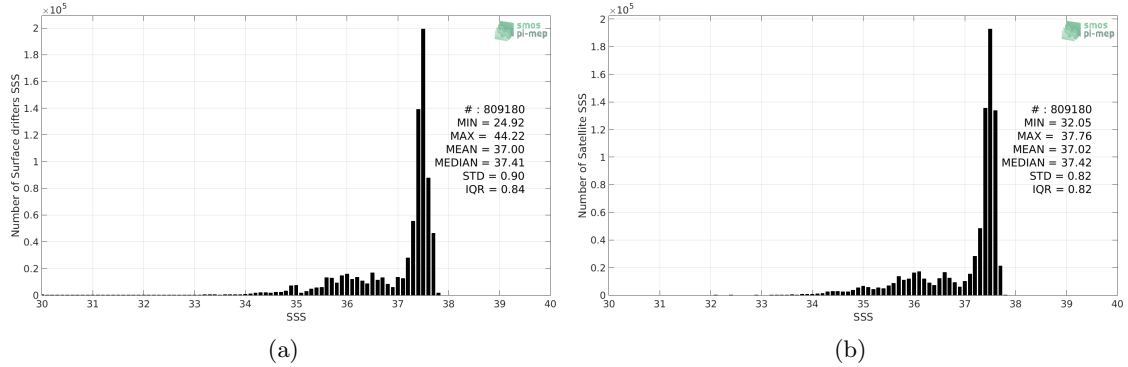
Figure 2: Histograms of SSS from Surface drifters (a) and SMAP SSS L4 OI v1 - Monthly (IPRC) (b) considering all match-up pairs per bins of 0.1 over the North Atlantic Ocean Pi-MEP region and for the full satellite product period.
