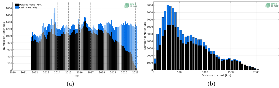
Figure 1: Number of match-ups between Argo and SMAP SSS L4 OI v1 - Monthly (IPRC) SSS as a function of time (a) and as function of the distance to coast (b) over the North Atlantic Ocean Pi-MEP region and for the full satellite product period.
