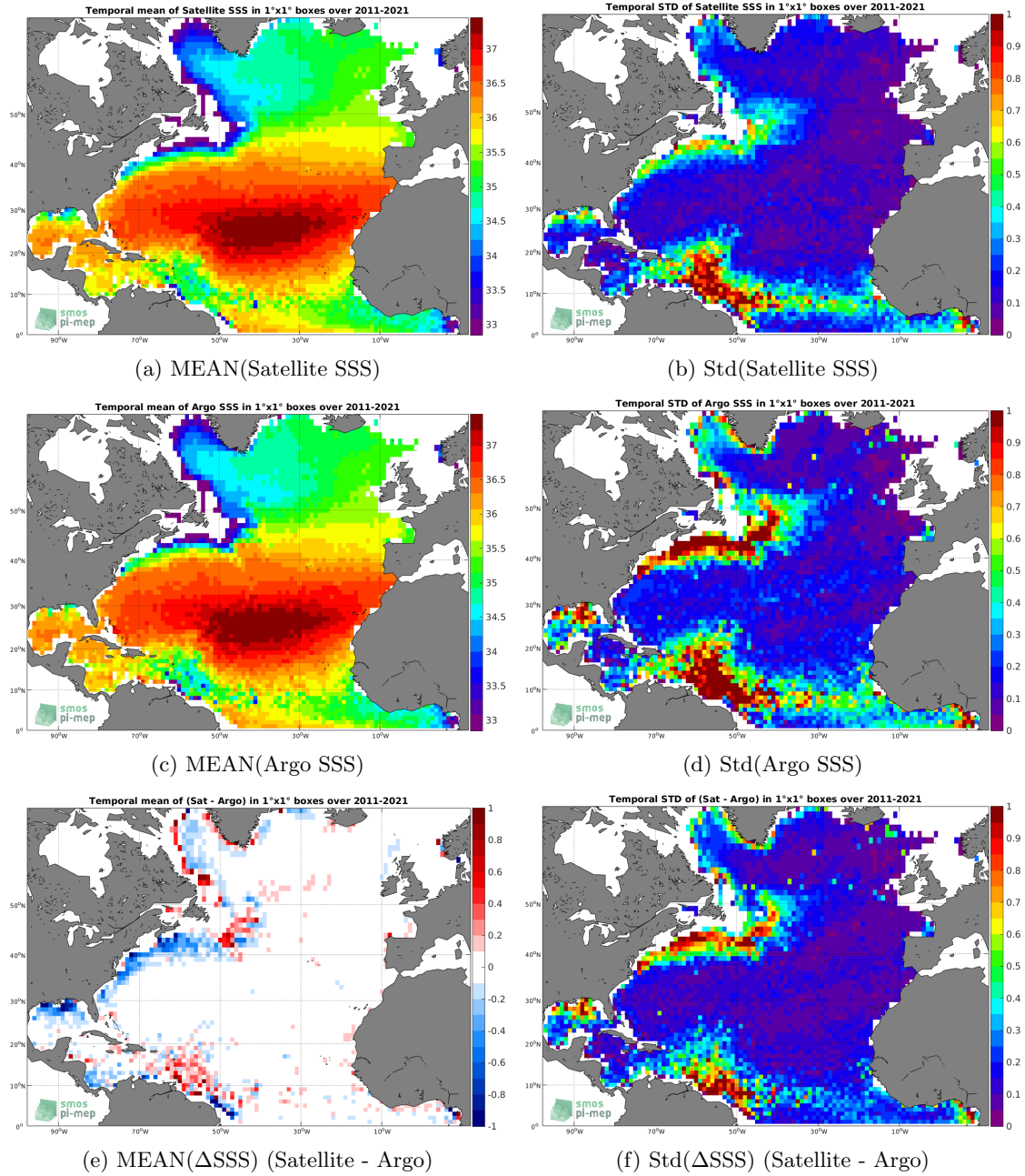
Figure 6: Temporal mean (left) and Std (right) of SSS from SMAP SSS L4 OI v1 - Monthly (IPRC) (top), Argo (middle), and of \Delta SSS (Satellite - Argo). Only match-up pairs are used to generate these maps.
