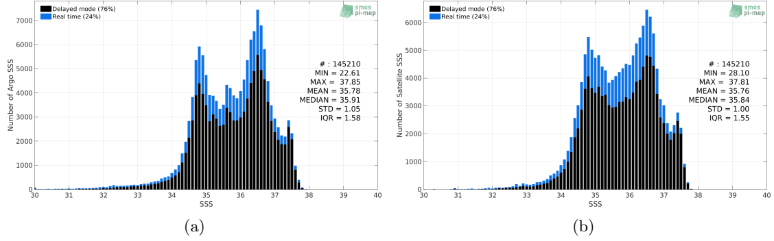
Figure 2: Histograms of SSS from Argo (a) and SMAP SSS L4 OI v1 - Monthly (IPRC) (b) considering all match-up pairs per bins of 0.1 over the North Atlantic Ocean Pi-MEP region and for the full satellite product period.
