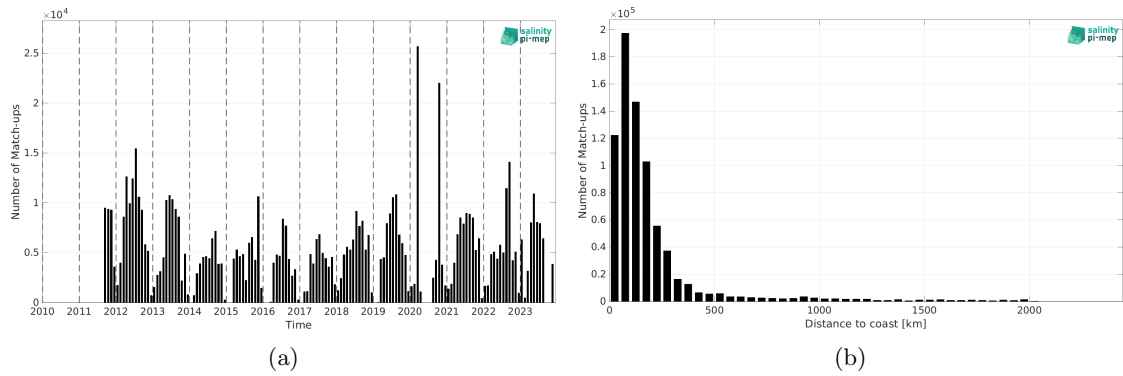
Figure 2: Number of match-ups between TSG (SAMOS) and SMAP SSS L4 OI v3 - Monthly (ESR) SSS as a function of time (a) and as function of the distance to coast (b) over the North Atlantic Ocean Pi-MEP region and for the full satellite product period.
