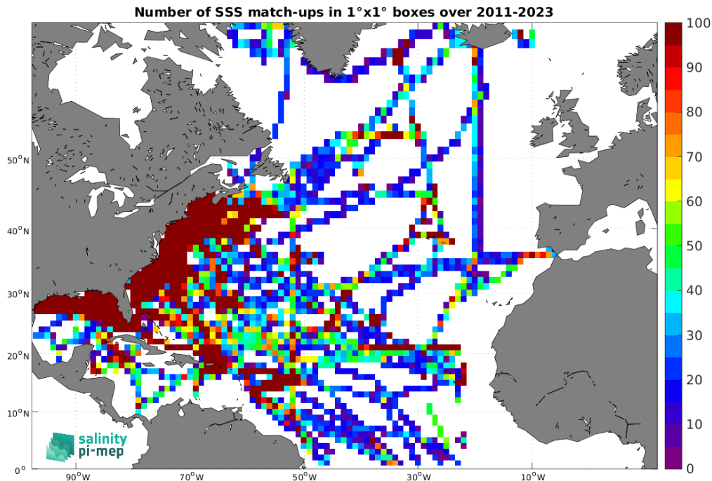
Figure 5: Number of SSS match-ups between TSG (SAMOS) SSS and the SMAP SSS L4 OI v3 - Monthly (ESR) SSS product for the North Atlantic Ocean Pi-MEP region over 1^\circ \times 1^\circ boxes and for the full satellite product period.
