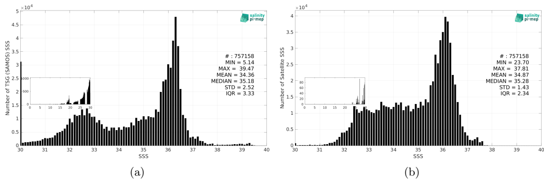
Figure 3: Histograms of SSS from TSG (SAMOS) (a) and SMAP SSS L4 OI v3 - Monthly (ESR) (b) considering all match-up pairs per bins of 0.1 over the North Atlantic Ocean Pi-MEP region and for the full satellite product period.
