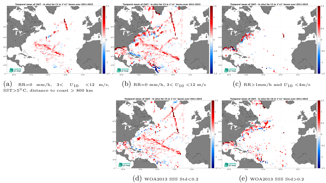
Figure 14: Temporal mean gridded over spatial boxes of size 1^\circ \times 1^\circ of \Delta\text{SSS} (SMAP SSS L4 OI v3 - Monthly (ESR) - TSG (SAMOS)) for 5 different subdatasets corresponding to:RR=0 mm/h, 3 < U_{10} < 12 m/s, SST > 5°C, distance to coast > 800 km (a), RR=0 mm/h, 3 < U_{10} < 12 m/s (b), RR > 1mm/h and U_{10} < 4 m/s (c), WOA2013 SSS Std < 0.2 (d), WOA2013 SSS Std > 0.2 (e).
