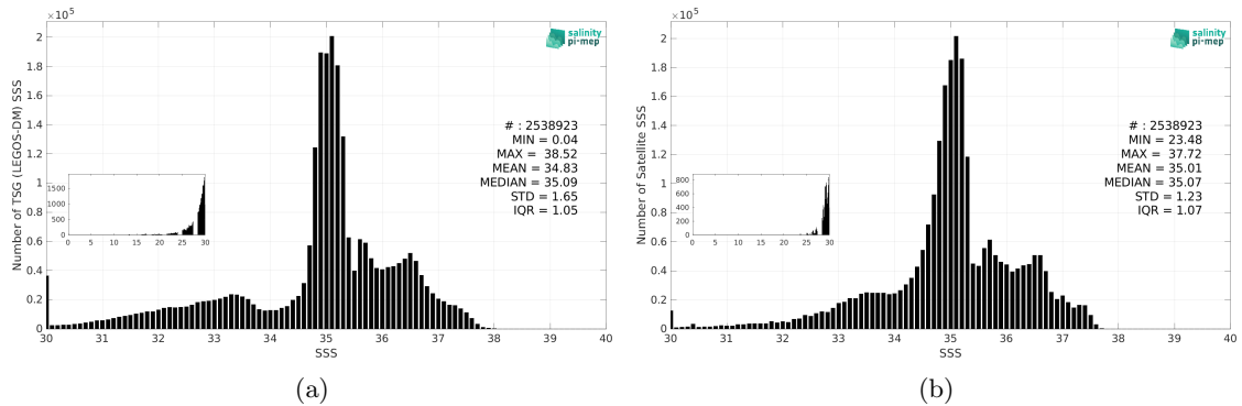
Figure 3: Histograms of SSS from TSG (LEGOS-DM) (a) and SMAP SSS L4 OI v3 - Monthly (ESR) (b) considering all match-up pairs per bins of 0.1 over the North Atlantic Ocean Pi-MEP region and for the full satellite product period.
