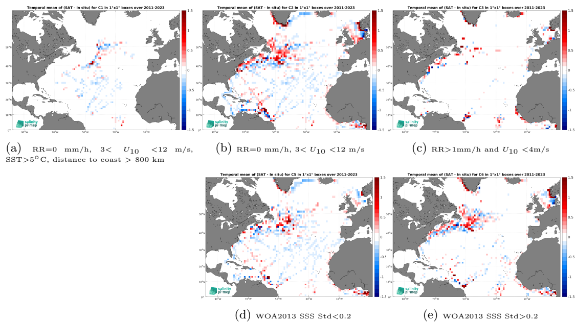
Figure 14: Temporal mean gridded over spatial boxes of size 1^\circ \times 1^\circ of \Delta\text{SSS} (SMAP SSS L4 OI v3 - Monthly (ESR) - TSG (LEGOS-DM)) for 5 different subdatasets corresponding to:RR=0 mm/h, 3 < U_{10} < 12 m/s, SST >5^\circ\text{C} , distance to coast > 800 km (a), RR=0 mm/h, 3 < U_{10} < 12 m/s (b), RR >1 mm/h and U_{10} < 4 m/s (c), WOA2013 SSS Std <0.2 (d), WOA2013 SSS Std >0.2 (e).
