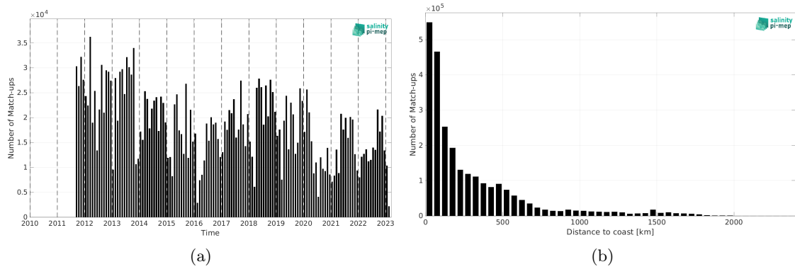
Figure 2: Number of match-ups between TSG (LEGOS-DM) and SMAP SSS L4 OI v3 - Monthly (ESR) SSS as a function of time (a) and as function of the distance to coast (b) over the North Atlantic Ocean Pi-MEP region and for the full satellite product period.
