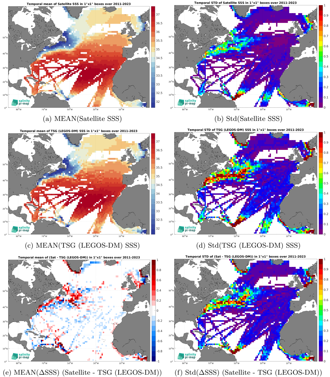
Figure 7: Temporal mean (left) and Std (right) of SSS from SMAP SSS L4 OI v3 - Monthly (ESR) (top), TSG (LEGOS-DM) (middle), and of \Delta SSS (Satellite - TSG (LEGOS-DM)). Only match-up pairs are used to generate these maps.
