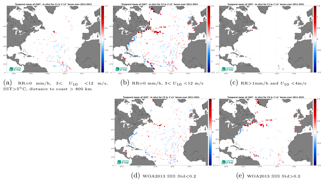
Figure 14: Temporal mean gridded over spatial boxes of size 1^\circ \times 1^\circ of \Delta\text{SSS} (SMAP SSS L4 OI v3 - Monthly (ESR) - TSG (GOSUD-Sailing-ship)) for 5 different subdatasets corresponding to:RR=0 mm/h, 3 < U_{10} < 12 m/s, SST > 5°C, distance to coast > 800 km (a), RR=0 mm/h, 3 < U_{10} < 12 m/s (b), RR > 1mm/h and U_{10} < 4 m/s (c), WOA2013 SSS Std < 0.2 (d), WOA2013 SSS Std > 0.2 (e).
