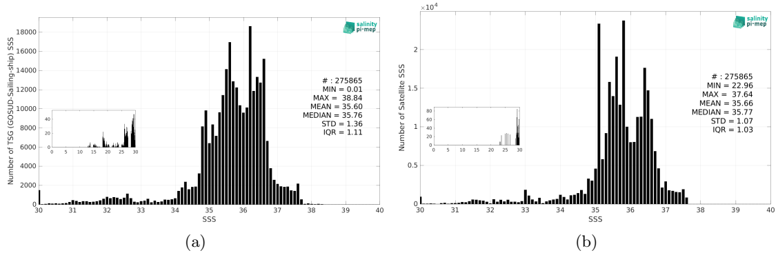
Figure 3: Histograms of SSS from TSG (GOSUD-Sailing-ship) (a) and SMAP SSS L4 OI v3 - Monthly (ESR) (b) considering all match-up pairs per bins of 0.1 over the North Atlantic Ocean Pi-MEP region and for the full satellite product period.
