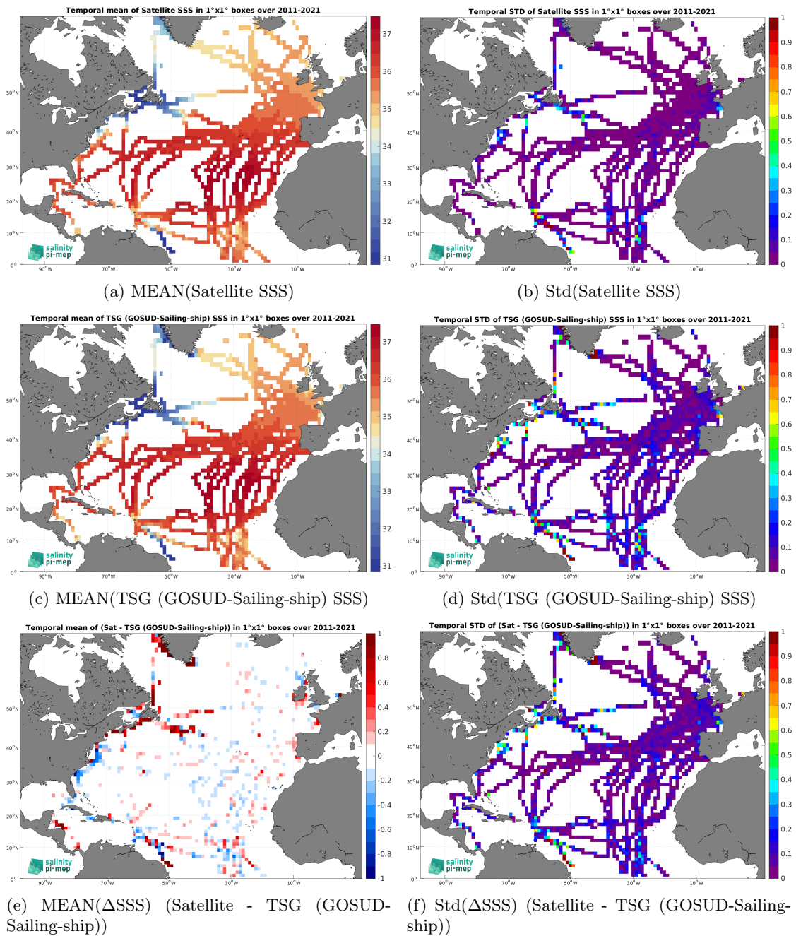
Figure 7: Temporal mean (left) and Std (right) of SSS from SMAP SSS L4 OI v3 - Monthly (ESR) (top), TSG (GOSUD-Sailing-ship) (middle), and of \Delta SSS (Satellite - TSG (GOSUD-Sailing-ship)). Only match-up pairs are used to generate these maps.
