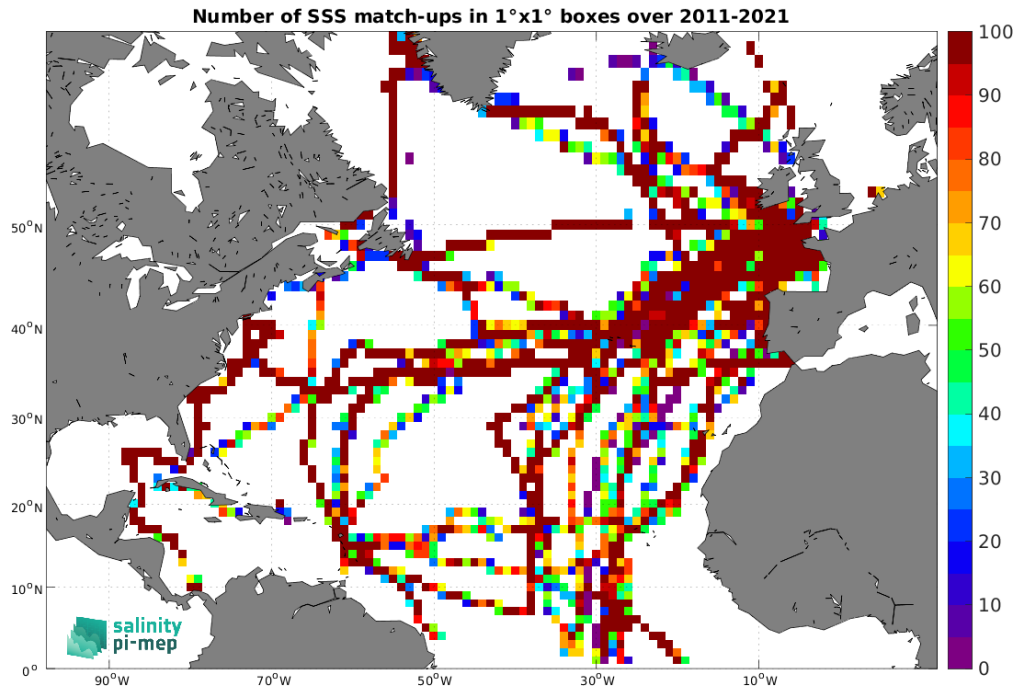
Figure 5: Number of SSS match-ups between TSG (GOSUD-Sailing-ship) SSS and the SMAP SSS L4 OI v3 - Monthly (ESR) SSS product for the North Atlantic Ocean Pi-MEP region over 1^\circ \times 1^\circ boxes and for the full satellite product period.
