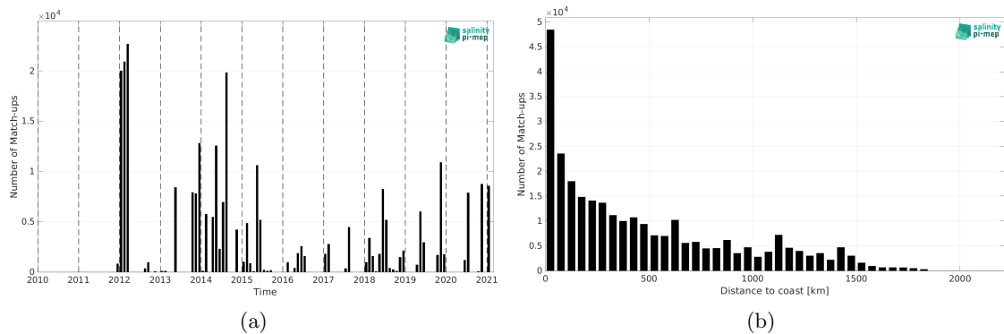
Figure 2: Number of match-ups between TSG (GOSUD-Sailing-ship) and SMAP SSS L4 OI v3 - Monthly (ESR) SSS as a function of time (a) and as function of the distance to coast (b) over the North Atlantic Ocean Pi-MEP region and for the full satellite product period.
