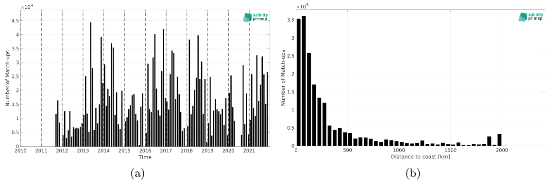
Figure 2: Number of match-ups between TSG (GOSUD-Research-vessel) and SMAP SSS L4 OI v3 - Monthly (ESR) SSS as a function of time (a) and as function of the distance to coast (b) over the North Atlantic Ocean Pi-MEP region and for the full satellite product period.
