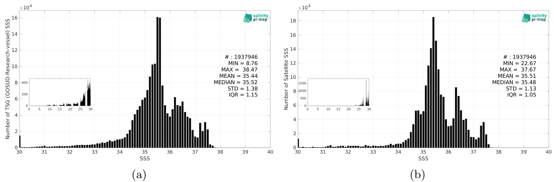
Figure 3: Histograms of SSS from TSG (GOSUD-Research-vessel) (a) and SMAP SSS L4 OI v3 - Monthly (ESR) (b) considering all match-up pairs per bins of 0.1 over the North Atlantic Ocean Pi-MEP region and for the full satellite product period.
