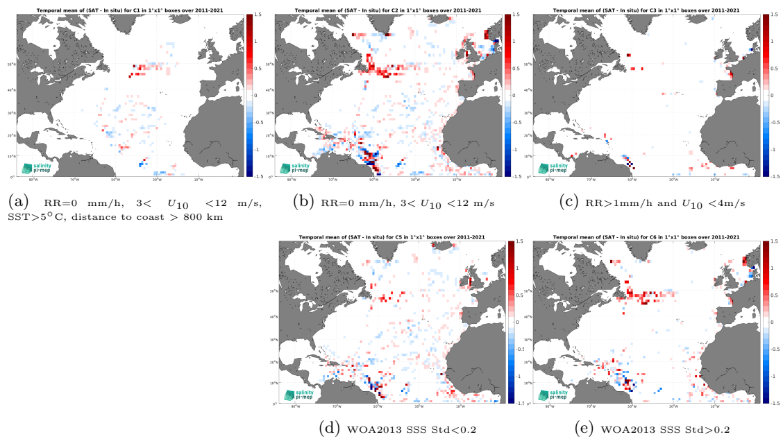
Figure 14: Temporal mean gridded over spatial boxes of size 1^\circ \times 1^\circ of \Delta\text{SSS} (SMAP SSS L4 OI v3 - Monthly (ESR) - TSG (GOSUD-Research-vessel)) for 5 different subdatasets corresponding to:RR=0 mm/h, 3 < U_{10} < 12 m/s, SST >5^\circ\text{C} , distance to coast > 800 km (a), RR=0 mm/h, 3 < U_{10} < 12 m/s (b), RR >1 mm/h and U_{10} < 4 m/s (c), WOA2013 SSS Std <0.2 (d), WOA2013 SSS Std >0.2 (e).
