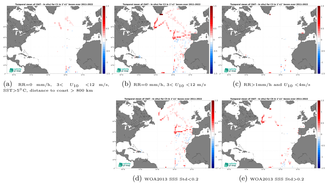
Figure 14: Temporal mean gridded over spatial boxes of size 1^\circ \times 1^\circ of \Delta\text{SSS} (SMAP SSS L4 OI v3 - Monthly (ESR) - TSG (CSIC-UTM)) for 5 different subdatasets corresponding to:RR=0 mm/h, 3 < U_{10} < 12 m/s, SST >5^\circ\text{C} , distance to coast > 800 km (a), RR=0 mm/h, 3 < U_{10} < 12 m/s (b), RR >1 mm/h and U_{10} < 4 m/s (c), WOA2013 SSS Std <0.2 (d), WOA2013 SSS Std >0.2 (e).
