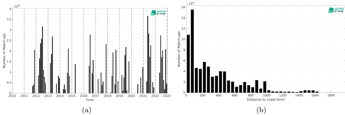
Figure 2: Number of match-ups between TSG (CSIC-UTM) and SMAP SSS L4 OI v3 - Monthly (ESR) SSS as a function of time (a) and as function of the distance to coast (b) over the North Atlantic Ocean Pi-MEP region and for the full satellite product period.
