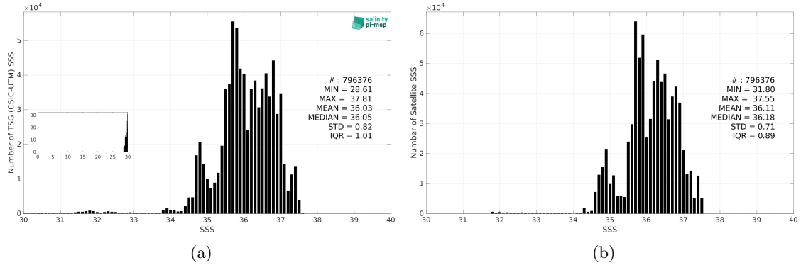
Figure 3: Histograms of SSS from TSG (CSIC-UTM) (a) and SMAP SSS L4 OI v3 - Monthly (ESR) (b) considering all match-up pairs per bins of 0.1 over the North Atlantic Ocean Pi-MEP region and for the full satellite product period.
