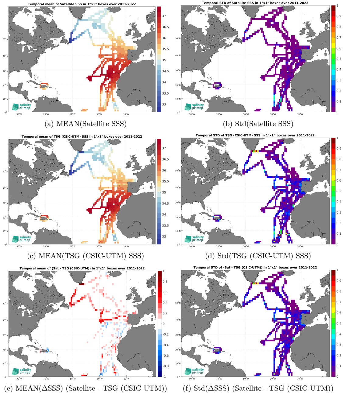
Figure 7: Temporal mean (left) and Std (right) of SSS from SMAP SSS L4 OI v3 - Monthly (ESR) (top), TSG (CSIC-UTM) (middle), and of \Delta SSS (Satellite - TSG (CSIC-UTM)). Only match-up pairs are used to generate these maps.
