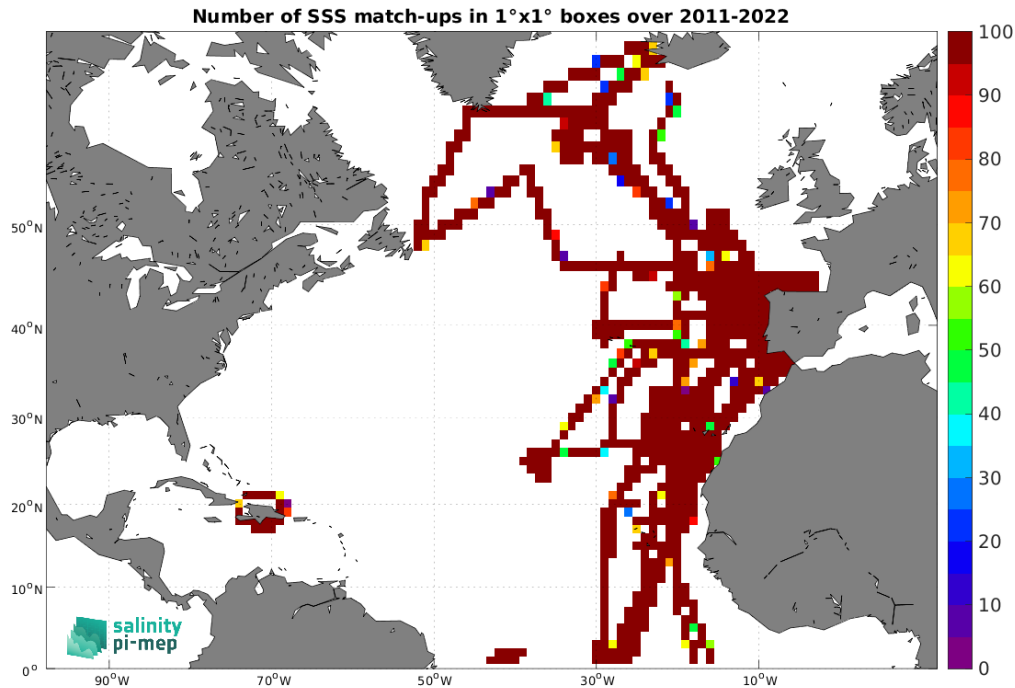
Figure 5: Number of SSS match-ups between TSG (CSIC-UTM) SSS and the SMAP SSS L4 OI v3 - Monthly (ESR) SSS product for the North Atlantic Ocean Pi-MEP region over 1^\circ \times 1^\circ boxes and for the full satellite product period.
