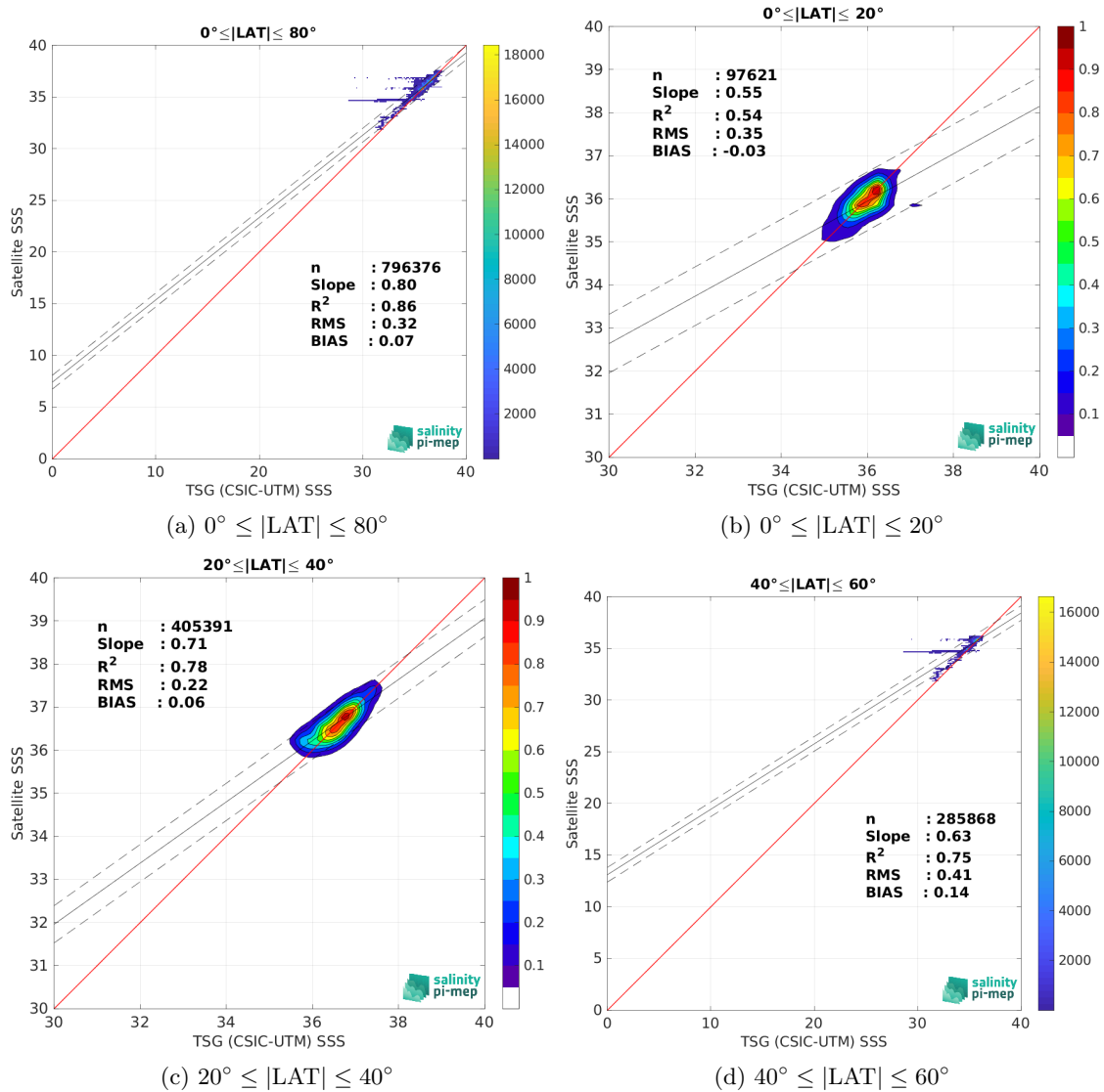
Figure 10: Contour maps of the concentration of SMAP SSS L4 OI v3 - Monthly (ESR) SSS (y-axis) versus TSG (CSIC-UTM) SSS (x-axis) at match-up pairs for different latitude bands. For each plot, the red line shows x=y . The black thin and dashed lines indicate a linear fit through the data cloud and the \pm 95\% confidence levels, respectively. The number match-up pairs n , the slope and R^2 coefficient of the linear fit, the root mean square (RMS) and the mean bias between satellite and in situ data are indicated for each latitude band in each plots.
