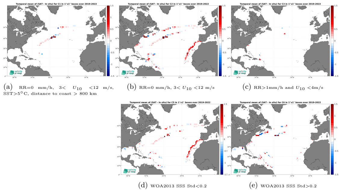
Figure 14: Temporal mean gridded over spatial boxes of size 1^\circ \times 1^\circ of \Delta\text{SSS} (SMAP SSS L4 OI v3 - Monthly (ESR) - Saildrone) for 5 different subdatasets corresponding to:RR=0 mm/h, 3 < U_{10} < 12 m/s, SST >5^\circ\text{C} , distance to coast > 800 km (a), RR=0 mm/h, 3 < U_{10} < 12 m/s (b), RR >1 mm/h and U_{10} < 4 m/s (c), WOA2013 SSS Std <0.2 (d), WOA2013 SSS Std >0.2 (e).
