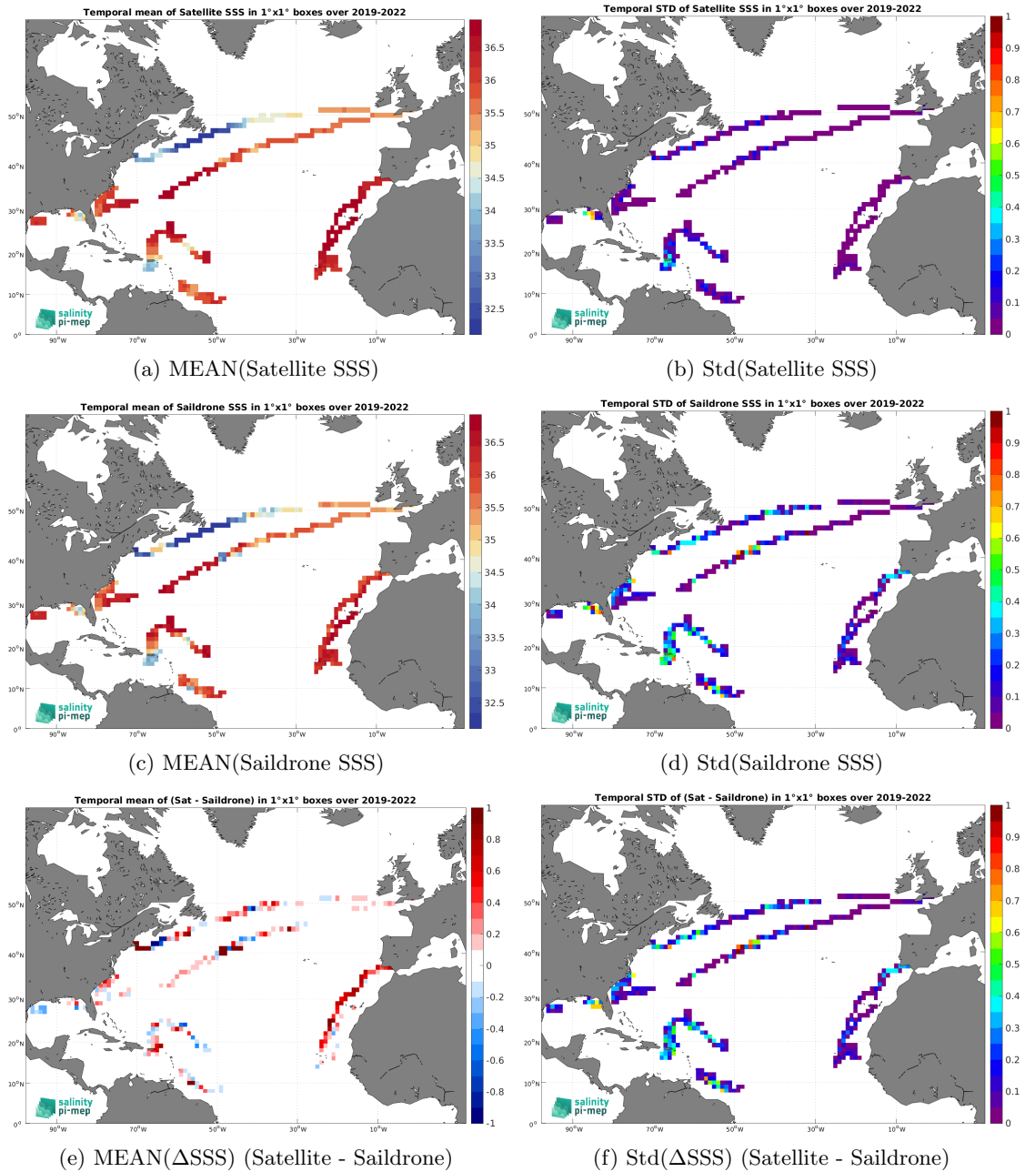
Figure 7: Temporal mean (left) and Std (right) of SSS from SMAP SSS L4 OI v3 - Monthly (ESR) (top), Saildrone (middle), and of \Delta SSS (Satellite - Saildrone). Only match-up pairs are used to generate these maps.
