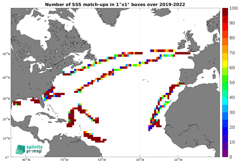
Figure 5: Number of SSS match-ups between Saildrone SSS and the SMAP SSS L4 OI v3 - Monthly (ESR) SSS product for the North Atlantic Ocean Pi-MEP region over 1^\circ \times 1^\circ boxes and for the full satellite product period.
