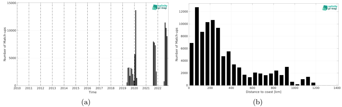
Figure 2: Number of match-ups between Saildrone and SMAP SSS L4 OI v3 - Monthly (ESR) SSS as a function of time (a) and as function of the distance to coast (b) over the North Atlantic Ocean Pi-MEP region and for the full satellite product period.
