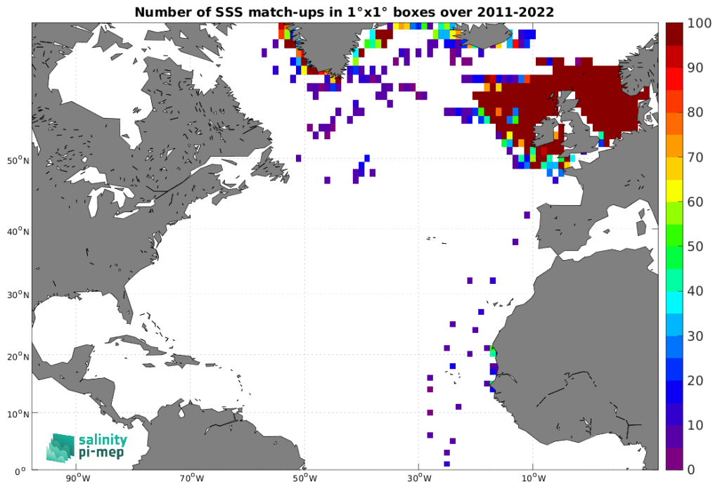
Figure 5: Number of SSS match-ups between ICES SSS and the SMAP SSS L4 OI v3 - Monthly (ESR) SSS product for the North Atlantic Ocean Pi-MEP region over 1°×1° boxes and for the full satellite product period.
