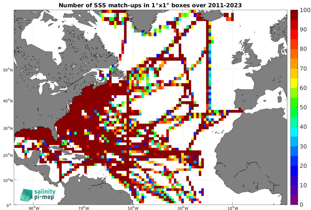
Figure 5: Number of SSS match-ups between TSG (SAMOS) SSS and the SMAP SSS L4 OI v3 - Daily (ESR) SSS product for the North Atlantic Ocean Pi-MEP region over 1^\circ \times 1^\circ boxes and for the full satellite product period.
