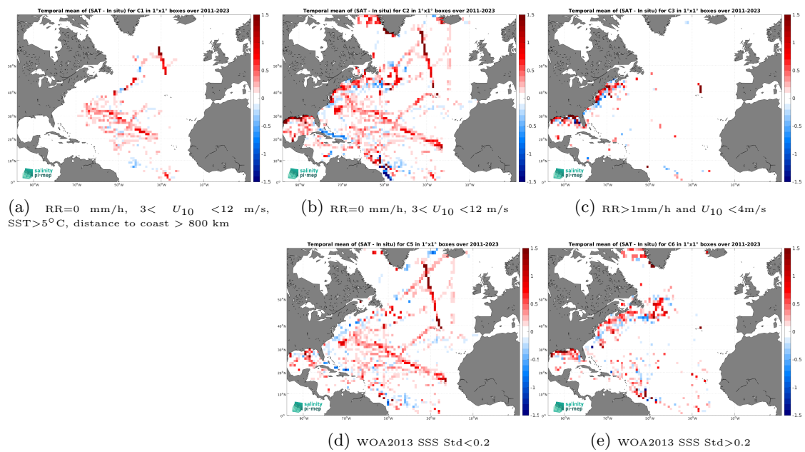
Figure 14: Temporal mean gridded over spatial boxes of size 1^\circ \times 1^\circ of \Delta\text{SSS} (SMAP SSS L4 OI v3 - Daily (ESR) - TSG (SAMOS)) for 5 different subdatasets corresponding to:RR=0 mm/h, 3 < U_{10} < 12 m/s, SST >5^\circ\text{C} , distance to coast > 800 km (a), RR=0 mm/h, 3 < U_{10} < 12 m/s (b), RR >1 mm/h and U_{10} < 4 m/s (c), WOA2013 SSS Std <0.2 (d), WOA2013 SSS Std >0.2 (e).
