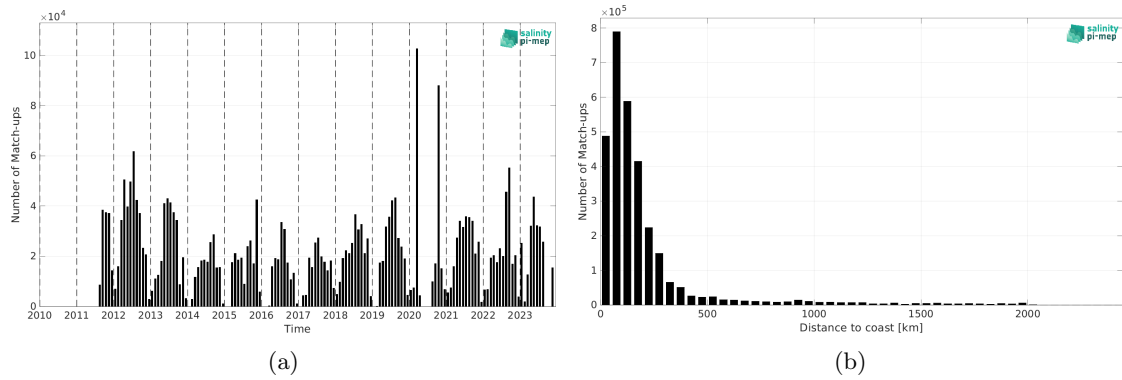
Figure 2: Number of match-ups between TSG (SAMOS) and SMAP SSS L4 OI v3 - Daily (ESR) SSS as a function of time (a) and as function of the distance to coast (b) over the North Atlantic Ocean Pi-MEP region and for the full satellite product period.
