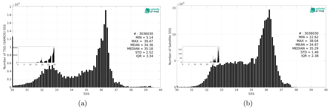
Figure 3: Histograms of SSS from TSG (SAMOS) (a) and SMAP SSS L4 OI v3 - Daily (ESR) (b) considering all match-up pairs per bins of 0.1 over the North Atlantic Ocean Pi-MEP region and for the full satellite product period.
