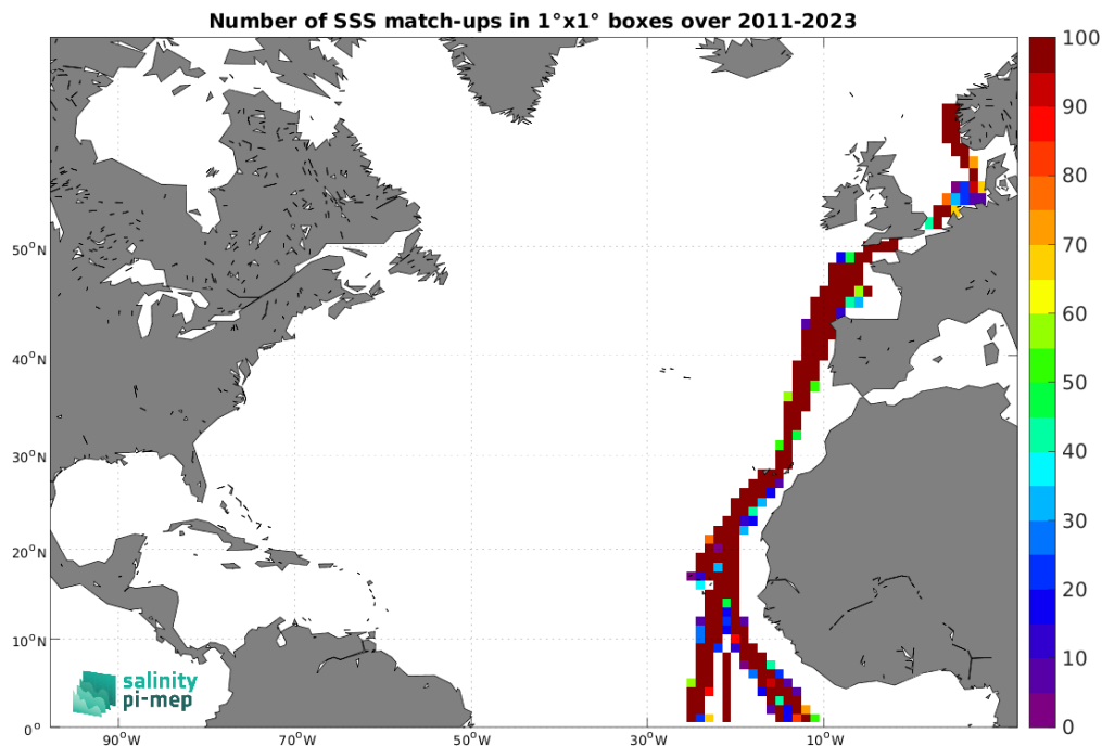
Figure 5: Number of SSS match-ups between TSG (Polarstern) SSS and the SMAP SSS L4 OI v3 - Daily (ESR) SSS product for the North Atlantic Ocean Pi-MEP region over 1^\circ \times 1^\circ boxes and for the full satellite product period.
