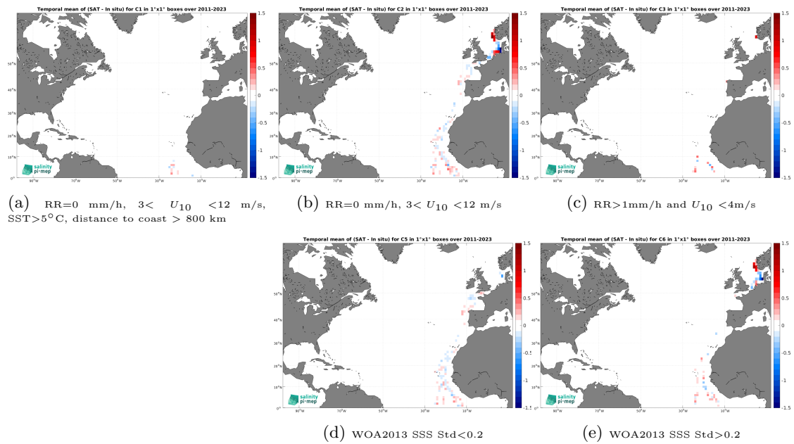
Figure 14: Temporal mean gridded over spatial boxes of size 1^\circ \times 1^\circ of \Delta\text{SSS} (SMAP SSS L4 OI v3 - Daily (ESR) - TSG (Polarstern)) for 5 different subdatasets corresponding to:RR=0 mm/h, 3 < U_{10} < 12 m/s, SST >5^\circ\text{C} , distance to coast > 800 km (a), RR=0 mm/h, 3 < U_{10} < 12 m/s (b), RR >1 mm/h and U_{10} < 4 m/s (c), WOA2013 SSS Std <0.2 (d), WOA2013 SSS Std >0.2 (e).
