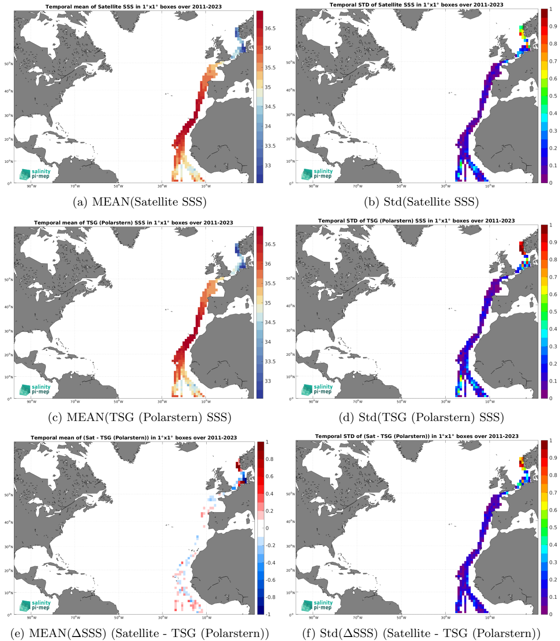
Figure 7: Temporal mean (left) and Std (right) of SSS from SMAP SSS L4 OI v3 - Daily (ESR) (top), TSG (Polarstern) (middle), and of \Delta SSS (Satellite - TSG (Polarstern)). Only match-up pairs are used to generate these maps.
