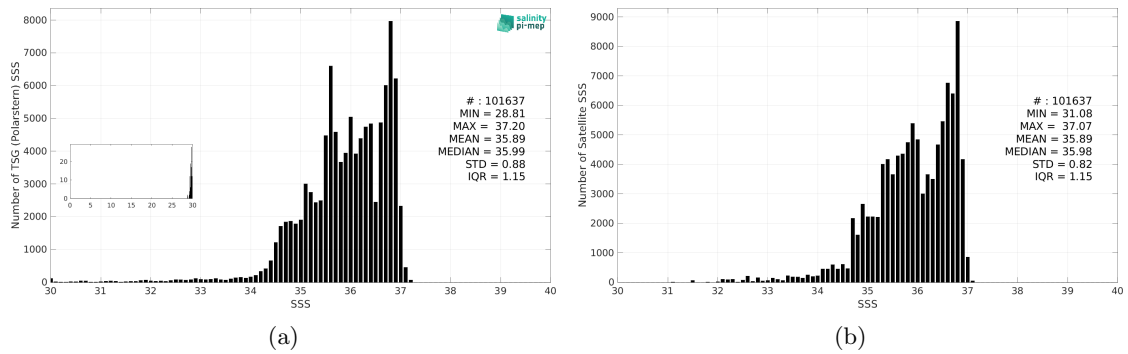
Figure 3: Histograms of SSS from TSG (Polarstern) (a) and SMAP SSS L4 OI v3 - Daily (ESR) (b) considering all match-up pairs per bins of 0.1 over the North Atlantic Ocean Pi-MEP region and for the full satellite product period.
