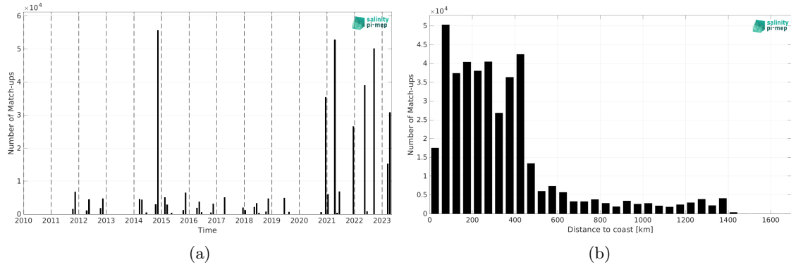
Figure 2: Number of match-ups between TSG (Polarstern) and SMAP SSS L4 OI v3 - Daily (ESR) SSS as a function of time (a) and as function of the distance to coast (b) over the North Atlantic Ocean Pi-MEP region and for the full satellite product period.
