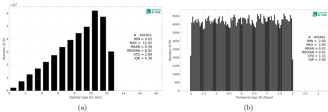
Figure 6: Histograms of the spatial (a) and temporal (b) lags between the location/time of the TSG (Polarstern) measurement and the date of the corresponding SMAP SSS L4 OI v3 - Daily (ESR) SSS pixel.
