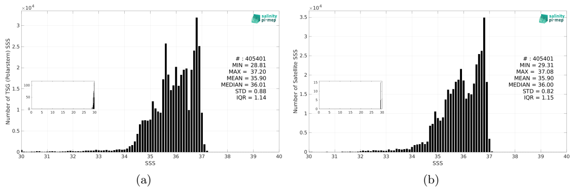
Figure 3: Histograms of SSS from TSG (Polarstern) (a) and SMAP SSS L4 OI v3 - Daily (ESR) (b) considering all match-up pairs per bins of 0.1 over the North Atlantic Ocean Pi-MEP region and for the full satellite product period.
