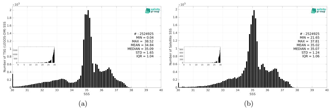
Figure 3: Histograms of SSS from TSG (LEGOS-DM) (a) and SMAP SSS L4 OI v3 - Daily (ESR) (b) considering all match-up pairs per bins of 0.1 over the North Atlantic Ocean Pi-MEP region and for the full satellite product period.
