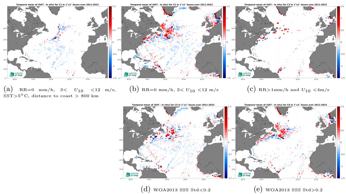
Figure 14: Temporal mean gridded over spatial boxes of size 1^\circ \times 1^\circ of \Delta\text{SSS} (SMAP SSS L4 OI v3 - Daily (ESR) - TSG (LEGOS-DM)) for 5 different subdatasets corresponding to:RR=0 mm/h, 3 < U_{10} < 12 m/s, SST >5^\circ\text{C} , distance to coast > 800 km (a), RR=0 mm/h, 3 < U_{10} < 12 m/s (b), RR >1 mm/h and U_{10} < 4 m/s (c), WOA2013 SSS Std <0.2 (d), WOA2013 SSS Std >0.2 (e).
