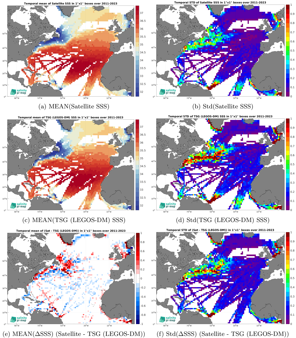
Figure 7: Temporal mean (left) and Std (right) of SSS from SMAP SSS L4 OI v3 - Daily (ESR) (top), TSG (LEGOS-DM) (middle), and of \Delta SSS (Satellite - TSG (LEGOS-DM)). Only match-up pairs are used to generate these maps.
