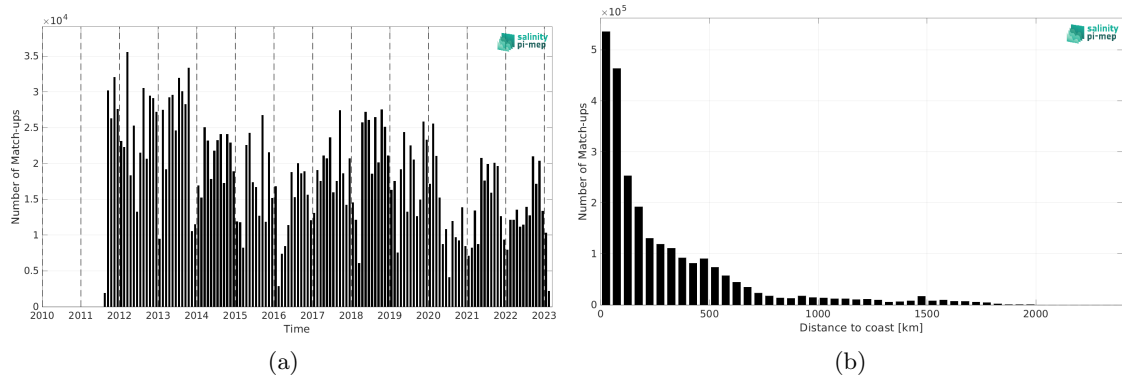
Figure 2: Number of match-ups between TSG (LEGOS-DM) and SMAP SSS L4 OI v3 - Daily (ESR) SSS as a function of time (a) and as function of the distance to coast (b) over the North Atlantic Ocean Pi-MEP region and for the full satellite product period.
