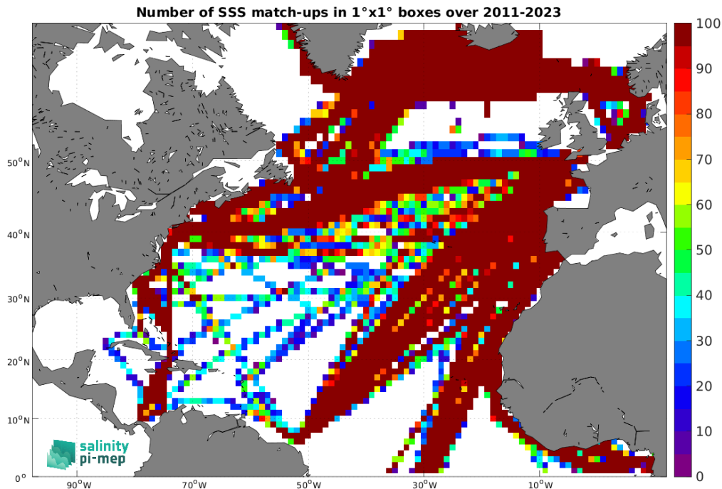
Figure 5: Number of SSS match-ups between TSG (LEGOS-DM) SSS and the SMAP SSS L4 OI v3 - Daily (ESR) SSS product for the North Atlantic Ocean Pi-MEP region over 1^\circ \times 1^\circ boxes and for the full satellite product period.
