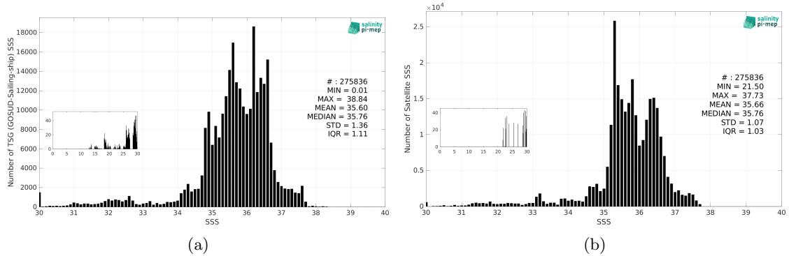
Figure 3: Histograms of SSS from TSG (GOSUD-Sailing-ship) (a) and SMAP SSS L4 OI v3 - Daily (ESR) (b) considering all match-up pairs per bins of 0.1 over the North Atlantic Ocean Pi-MEP region and for the full satellite product period.
