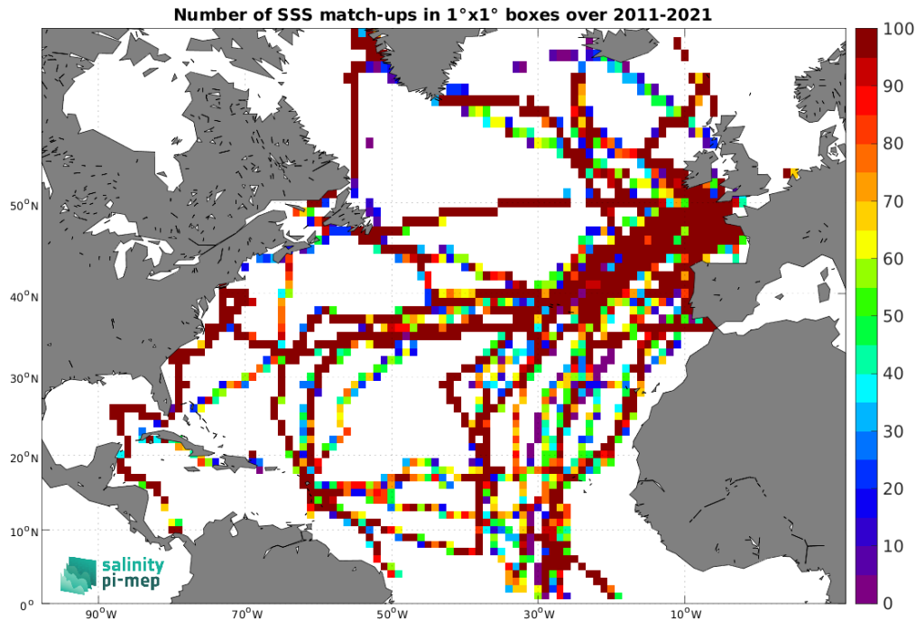
Figure 5: Number of SSS match-ups between TSG (GOSUD-Sailing-ship) SSS and the SMAP SSS L4 OI v3 - Daily (ESR) SSS product for the North Atlantic Ocean Pi-MEP region over 1^\circ \times 1^\circ boxes and for the full satellite product period.
