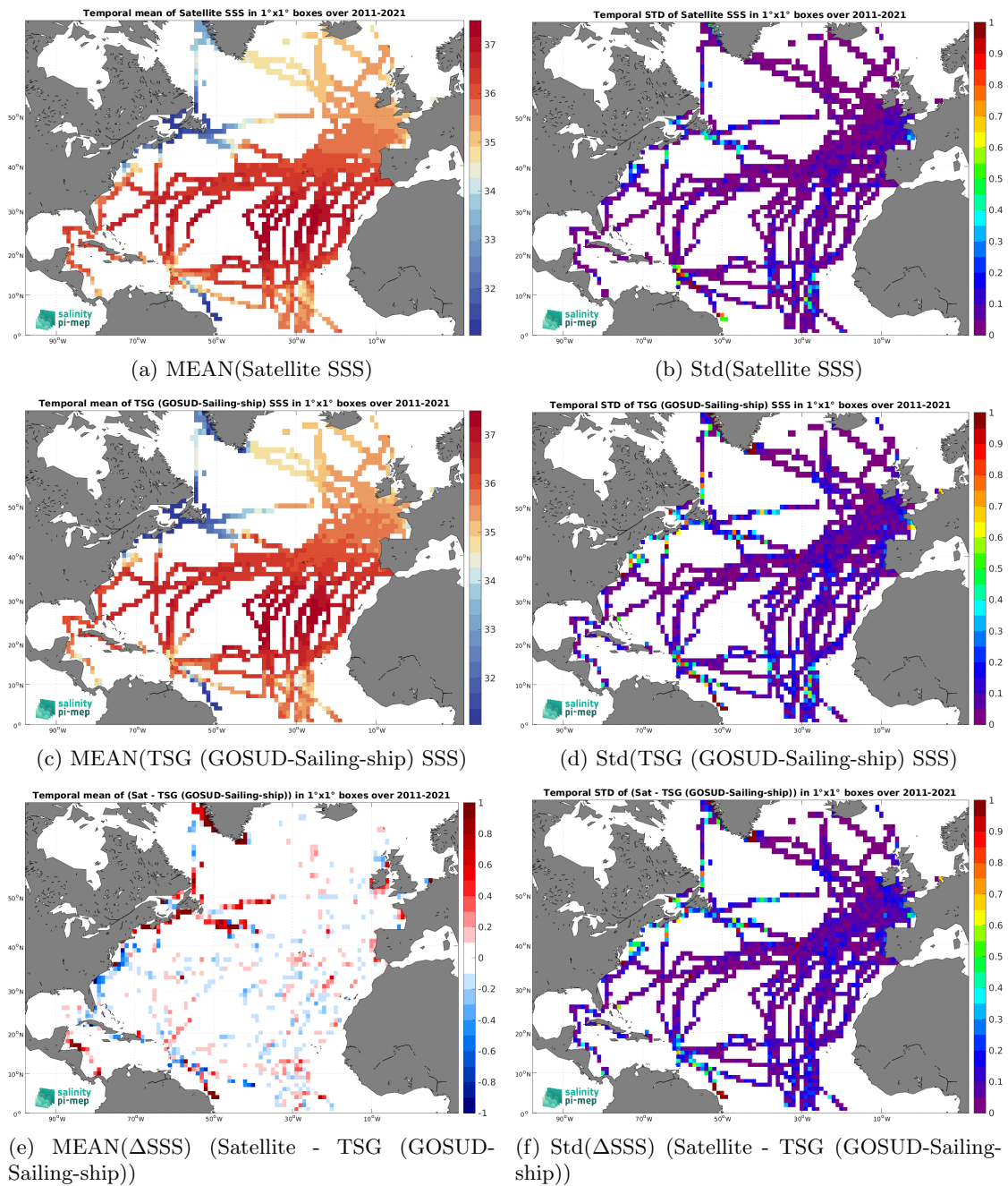
Figure 7: Temporal mean (left) and Std (right) of SSS from SMAP SSS L4 OI v3 - Daily (ESR) (top), TSG (GOSUD-Sailing-ship) (middle), and of \Delta SSS (Satellite - TSG (GOSUD-Sailing-ship)). Only match-up pairs are used to generate these maps.
