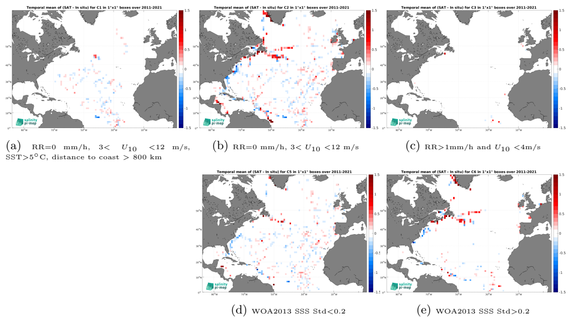
Figure 14: Temporal mean gridded over spatial boxes of size 1^\circ \times 1^\circ of \Delta\text{SSS} (SMAP SSS L4 OI v3 - Daily (ESR) - TSG (GOSUD-Sailing-ship)) for 5 different subdatasets corresponding to:RR=0 mm/h, 3 < U_{10} < 12 m/s, SST >5^\circ\text{C} , distance to coast > 800 km (a), RR=0 mm/h, 3 < U_{10} < 12 m/s (b), RR >1 mm/h and U_{10} < 4 m/s (c), WOA2013 SSS Std <0.2 (d), WOA2013 SSS Std >0.2 (e).
