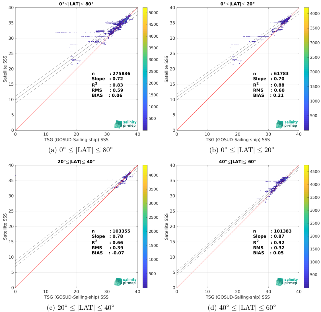
Figure 10: Contour maps of the concentration of SMAP SSS L4 OI v3 - Daily (ESR) SSS (y-axis) versus TSG (GOSUD-Sailing-ship) SSS (x-axis) at match-up pairs for different latitude bands. For each plot, the red line shows x=y . The black thin and dashed lines indicate a linear fit through the data cloud and the \pm 95\% confidence levels, respectively. The number match-up pairs n , the slope and R^2 coefficient of the linear fit, the root mean square (RMS) and the mean bias between satellite and in situ data are indicated for each latitude band in each plots.
