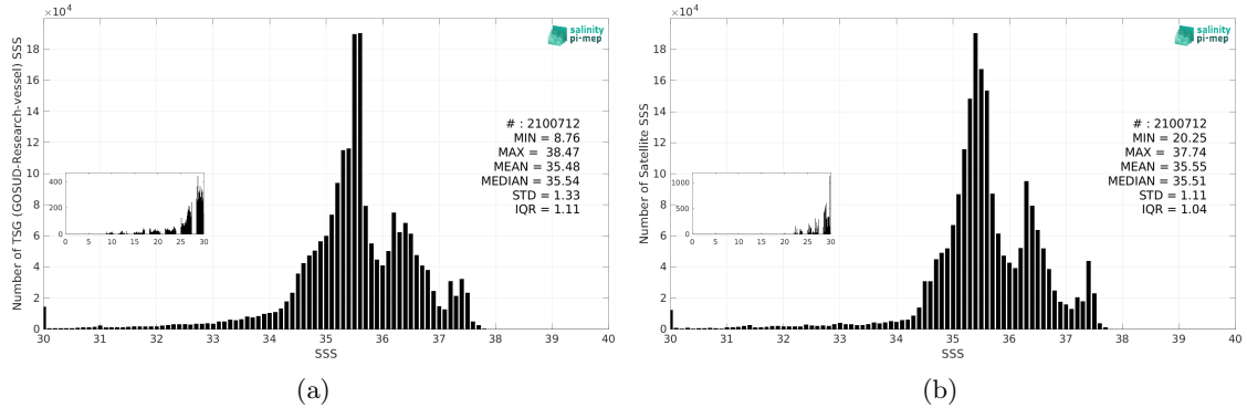
Figure 3: Histograms of SSS from TSG (GOSUD-Research-vessel) (a) and SMAP SSS L4 OI v3 - Daily (ESR) (b) considering all match-up pairs per bins of 0.1 over the North Atlantic Ocean Pi-MEP region and for the full satellite product period.
