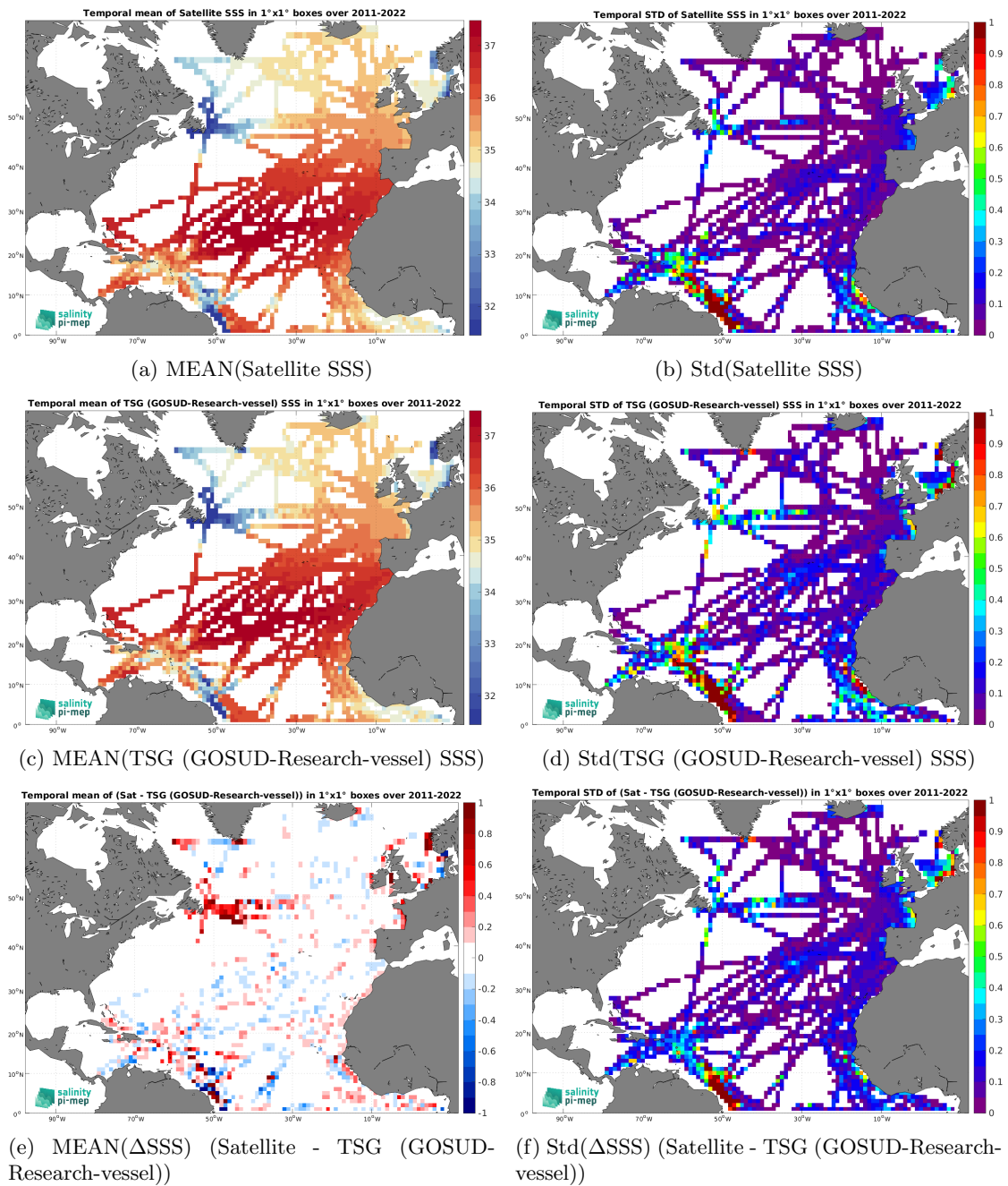
Figure 7: Temporal mean (left) and Std (right) of SSS from SMAP SSS L4 OI v3 - Daily (ESR) (top), TSG (GOSUD-Research-vessel) (middle), and of \Delta SSS (Satellite - TSG (GOSUD-Research-vessel)). Only match-up pairs are used to generate these maps.
