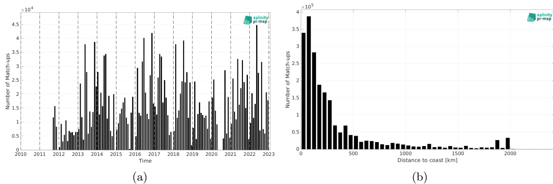
Figure 2: Number of match-ups between TSG (GOSUD-Research-vessel) and SMAP SSS L4 OI v3 - Daily (ESR) SSS as a function of time (a) and as function of the distance to coast (b) over the North Atlantic Ocean Pi-MEP region and for the full satellite product period.
