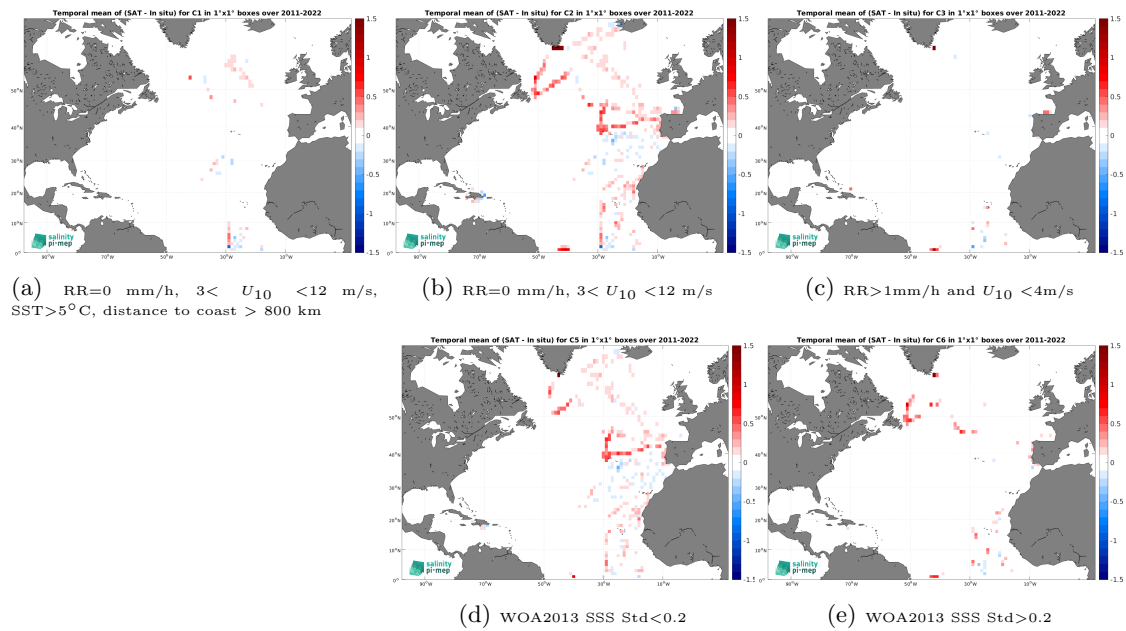
Figure 14: Temporal mean gridded over spatial boxes of size 1^\circ \times 1^\circ of \Delta\text{SSS} (SMAP SSS L4 OI v3 - Daily (ESR) - TSG (CSIC-UTM)) for 5 different subdatasets corresponding to:RR=0 mm/h, 3 < U_{10} < 12 m/s, SST > 5°C, distance to coast > 800 km (a), RR=0 mm/h, 3 < U_{10} < 12 m/s (b), RR > 1mm/h and U_{10} < 4 m/s (c), WOA2013 SSS Std < 0.2 (d), WOA2013 SSS Std > 0.2 (e).
