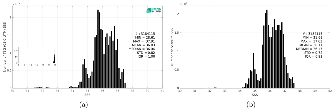
Figure 3: Histograms of SSS from TSG (CSIC-UTM) (a) and SMAP SSS L4 OI v3 - Daily (ESR) (b) considering all match-up pairs per bins of 0.1 over the North Atlantic Ocean Pi-MEP region and for the full satellite product period.
