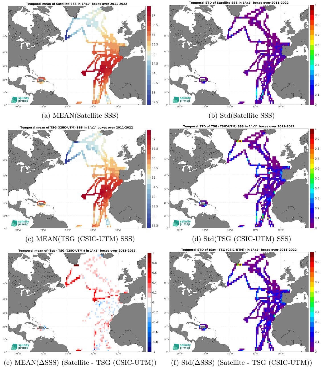
Figure 7: Temporal mean (left) and Std (right) of SSS from SMAP SSS L4 OI v3 - Daily (ESR) (top), TSG (CSIC-UTM) (middle), and of \Delta SSS (Satellite - TSG (CSIC-UTM)). Only match-up pairs are used to generate these maps.
