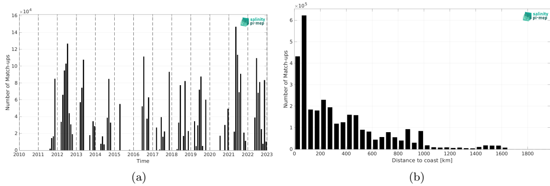
Figure 2: Number of match-ups between TSG (CSIC-UTM) and SMAP SSS L4 OI v3 - Daily (ESR) SSS as a function of time (a) and as function of the distance to coast (b) over the North Atlantic Ocean Pi-MEP region and for the full satellite product period.
