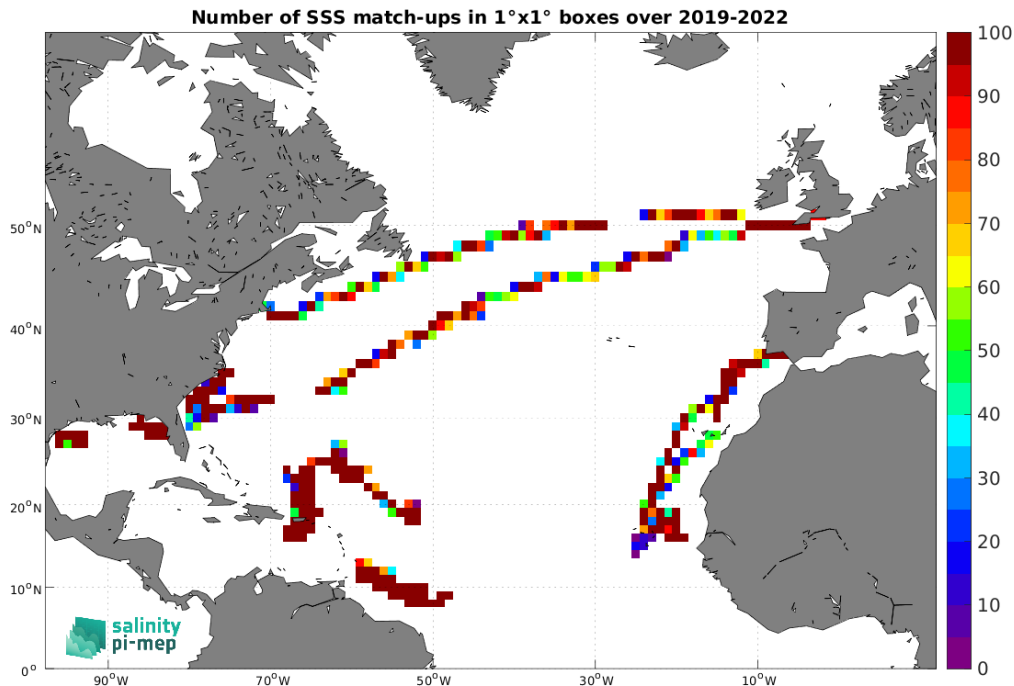
Figure 5: Number of SSS match-ups between Saildrone SSS and the SMAP SSS L4 OI v3 - Daily (ESR) SSS product for the North Atlantic Ocean Pi-MEP region over 1^\circ \times 1^\circ boxes and for the full satellite product period.
