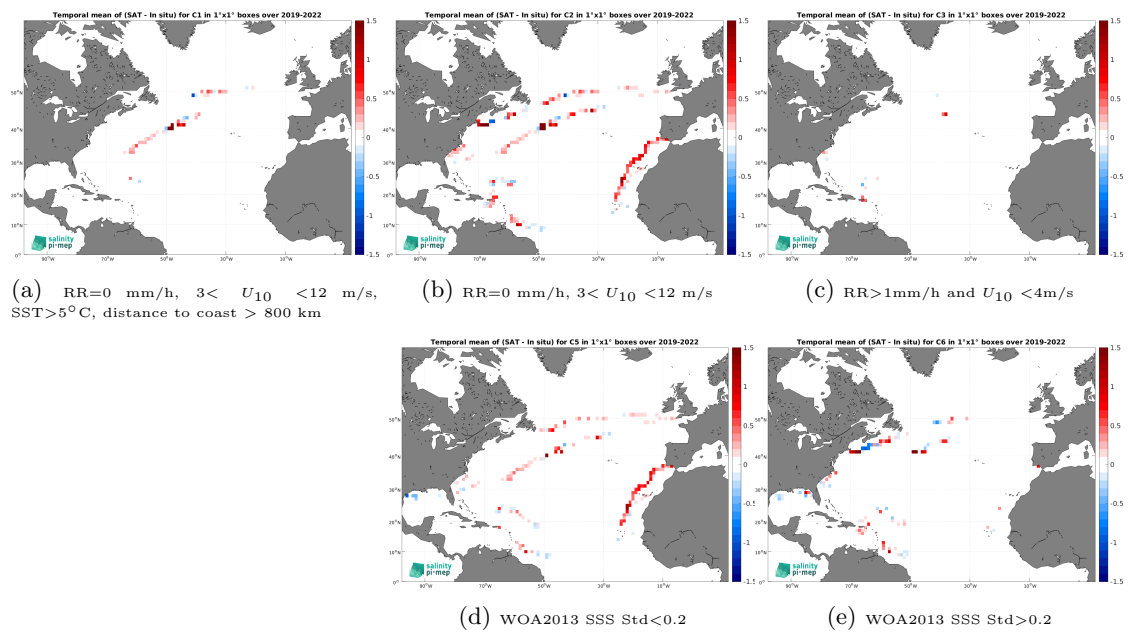
Figure 14: Temporal mean gridded over spatial boxes of size 1^\circ \times 1^\circ of \Delta\text{SSS} (SMAP SSS L4 OI v3 - Daily (ESR) - Saildrone) for 5 different subdatasets corresponding to:RR=0 mm/h, 3 < U_{10} < 12 m/s, SST > 5°C, distance to coast > 800 km (a), RR=0 mm/h, 3 < U_{10} < 12 m/s (b), RR > 1mm/h and U_{10} < 4 m/s (c), WOA2013 SSS Std < 0.2 (d), WOA2013 SSS Std > 0.2 (e).
