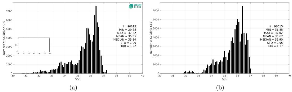
Figure 3: Histograms of SSS from Saildrone (a) and SMAP SSS L4 OI v3 - Daily (ESR) (b) considering all match-up pairs per bins of 0.1 over the North Atlantic Ocean Pi-MEP region and for the full satellite product period.
