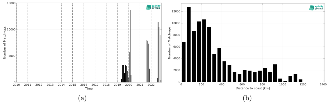
Figure 2: Number of match-ups between Saildrone and SMAP SSS L4 OI v3 - Daily (ESR) SSS as a function of time (a) and as function of the distance to coast (b) over the North Atlantic Ocean Pi-MEP region and for the full satellite product period.
