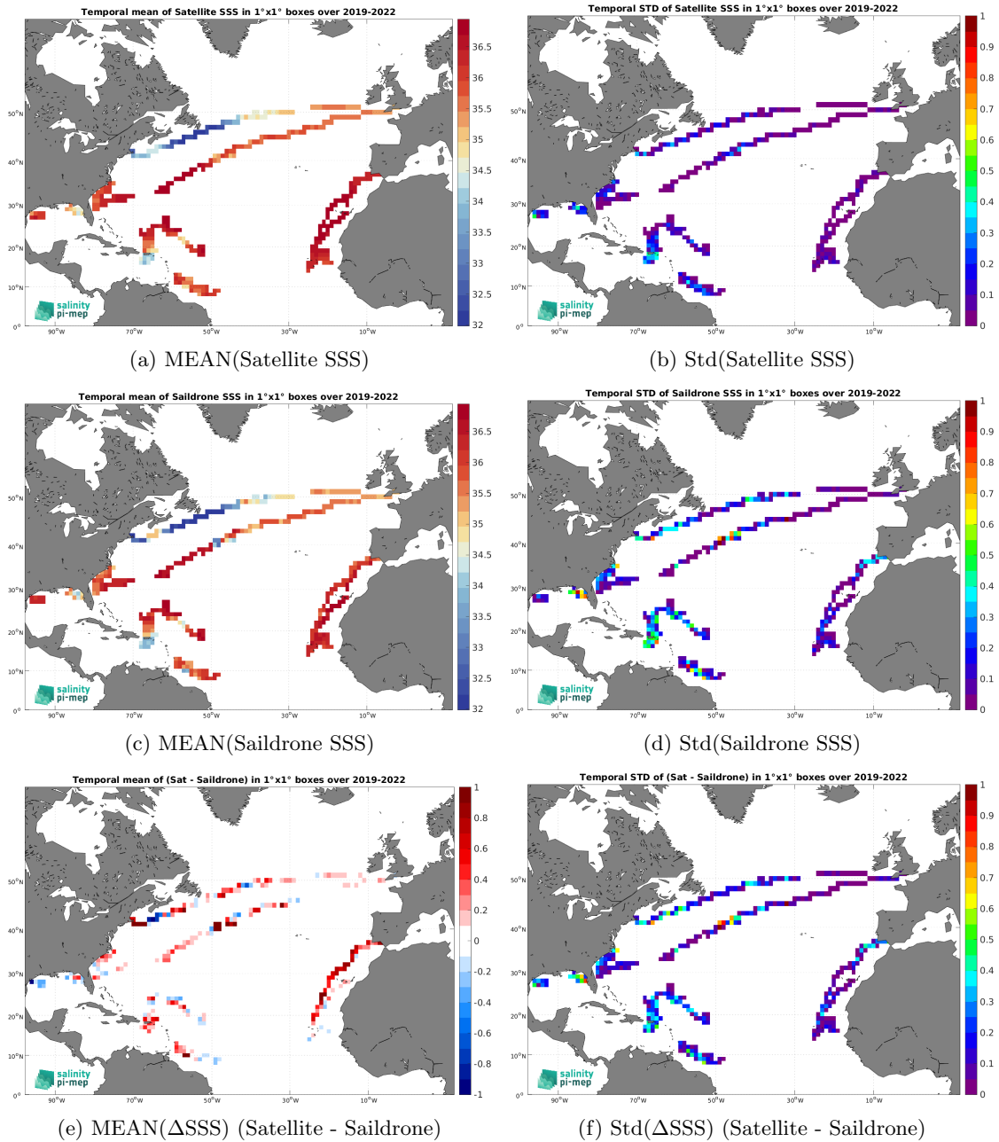
Figure 7: Temporal mean (left) and Std (right) of SSS from SMAP SSS L4 OI v3 - Daily (ESR) (top), Saildrone (middle), and of \Delta SSS (Satellite - Saildrone). Only match-up pairs are used to generate these maps.
