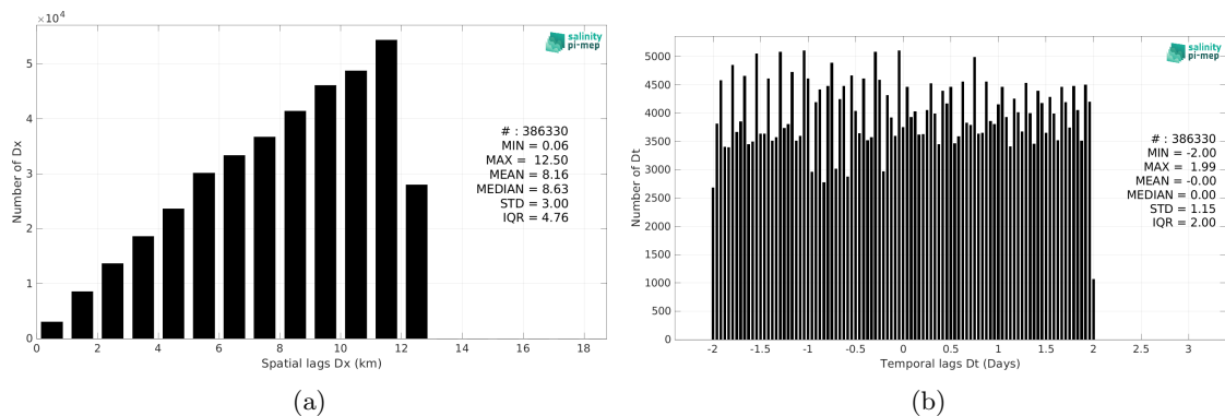
Figure 6: Histograms of the spatial (a) and temporal (b) lags between the location/time of the Saildrone measurements and the date of the corresponding SMAP SSS L4 OI v3 - Daily (ESR) SSS pixel.
