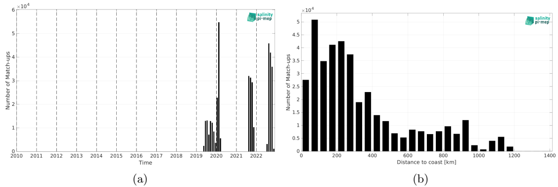
Figure 2: Number of match-ups between Saildrone and SMAP SSS L4 OI v3 - Daily (ESR) SSS as a function of time (a) and as function of the distance to coast (b) over the North Atlantic Ocean Pi-MEP region and for the full satellite product period.
