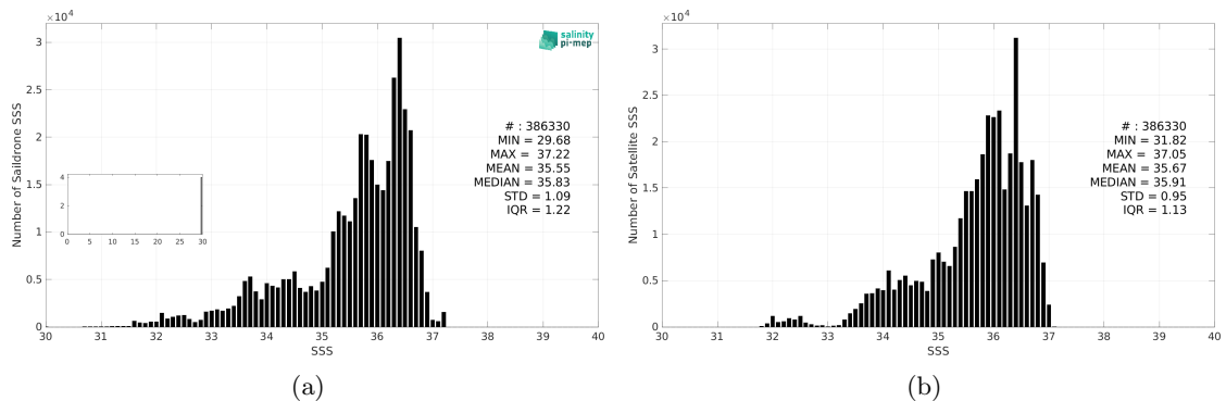
Figure 3: Histograms of SSS from Saildrone (a) and SMAP SSS L4 OI v3 - Daily (ESR) (b) considering all match-up pairs per bins of 0.1 over the North Atlantic Ocean Pi-MEP region and for the full satellite product period.
