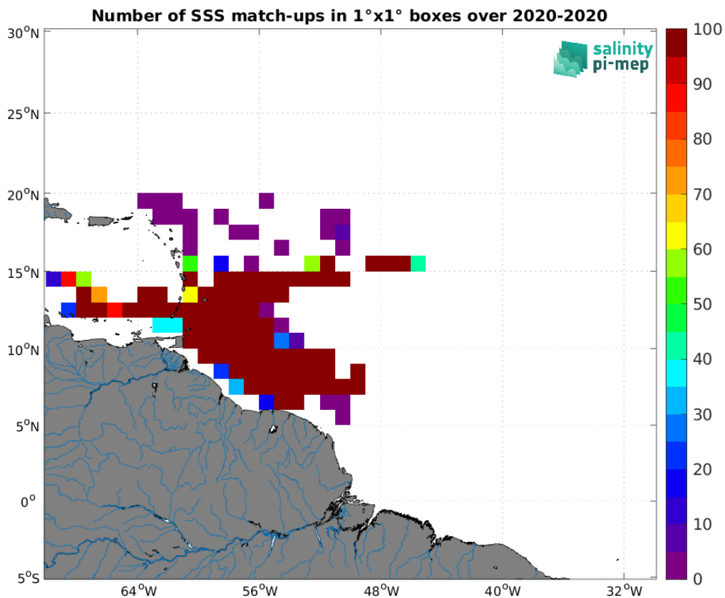
Figure 5: Number of SSS match-ups between EUREC4A SSS and the SMAP SSS L4 OI v3 - Daily (ESR) SSS product for the North Atlantic Ocean Pi-MEP region over 1^\circ \times 1^\circ boxes and for the full satellite product period.
