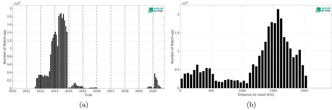
Figure 2: Number of match-ups between Surface drifters and SMAP SSS L4 OI v3 - Daily (ESR) SSS as a function of time (a) and as function of the distance to coast (b) over the North Atlantic Ocean Pi-MEP region and for the full satellite product period.
