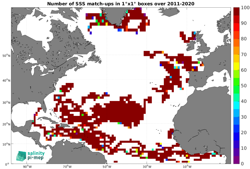
Figure 4: Number of SSS match-ups between Surface drifters SSS and the SMAP SSS L4 OI v3 - Daily (ESR) SSS product for the North Atlantic Ocean Pi-MEP region over 1^\circ \times 1^\circ boxes and for the full satellite product period.
