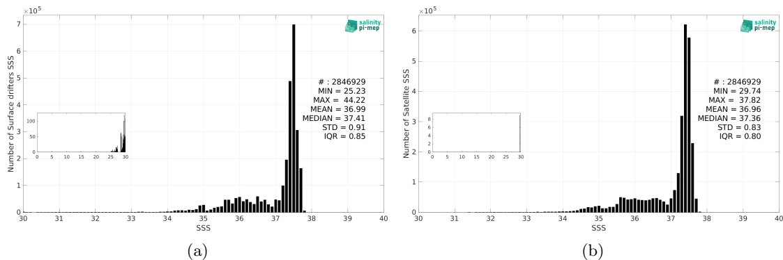
Figure 3: Histograms of SSS from Surface drifters (a) and SMAP SSS L4 OI v3 - Daily (ESR) (b) considering all match-up pairs per bins of 0.1 over the North Atlantic Ocean Pi-MEP region and for the full satellite product period.
