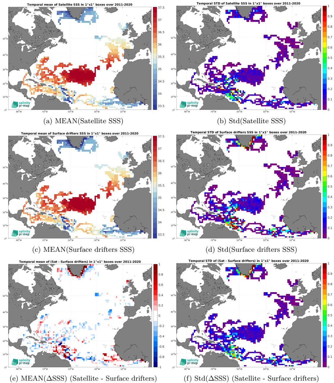
Figure 6: Temporal mean (left) and Std (right) of SSS from SMAP SSS L4 OI v3 - Daily (ESR) (top), Surface drifters (middle), and of \Delta SSS (Satellite - Surface drifters). Only match-up pairs are used to generate these maps.
