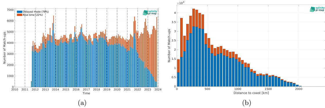
Figure 2: Number of match-ups between Argo and SMAP SSS L4 OI v3 - Daily (ESR) SSS as a function of time (a) and as function of the distance to coast (b) over the North Atlantic Ocean Pi-MEP region and for the full satellite product period.
