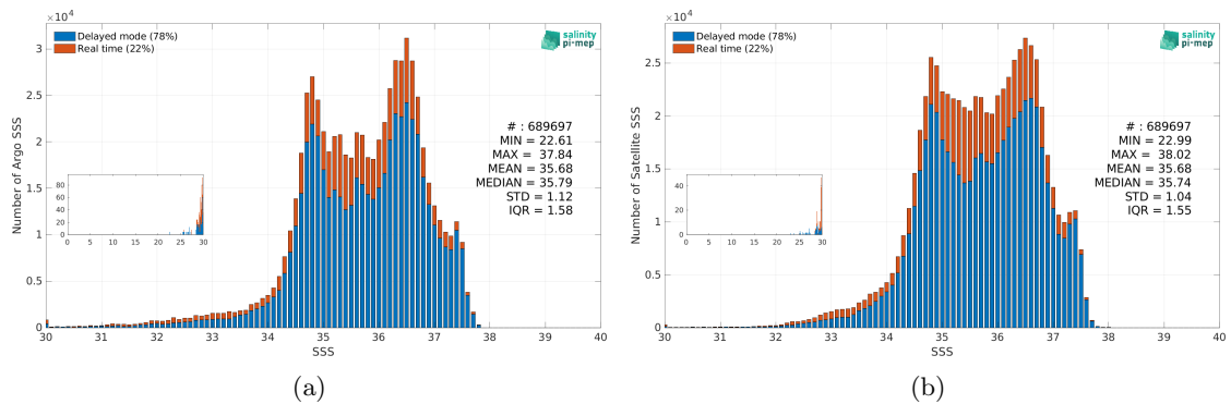
Figure 3: Histograms of SSS from Argo (a) and SMAP SSS L4 OI v3 - Daily (ESR) (b) considering all match-up pairs per bins of 0.1 over the North Atlantic Ocean Pi-MEP region and for the full satellite product period.
