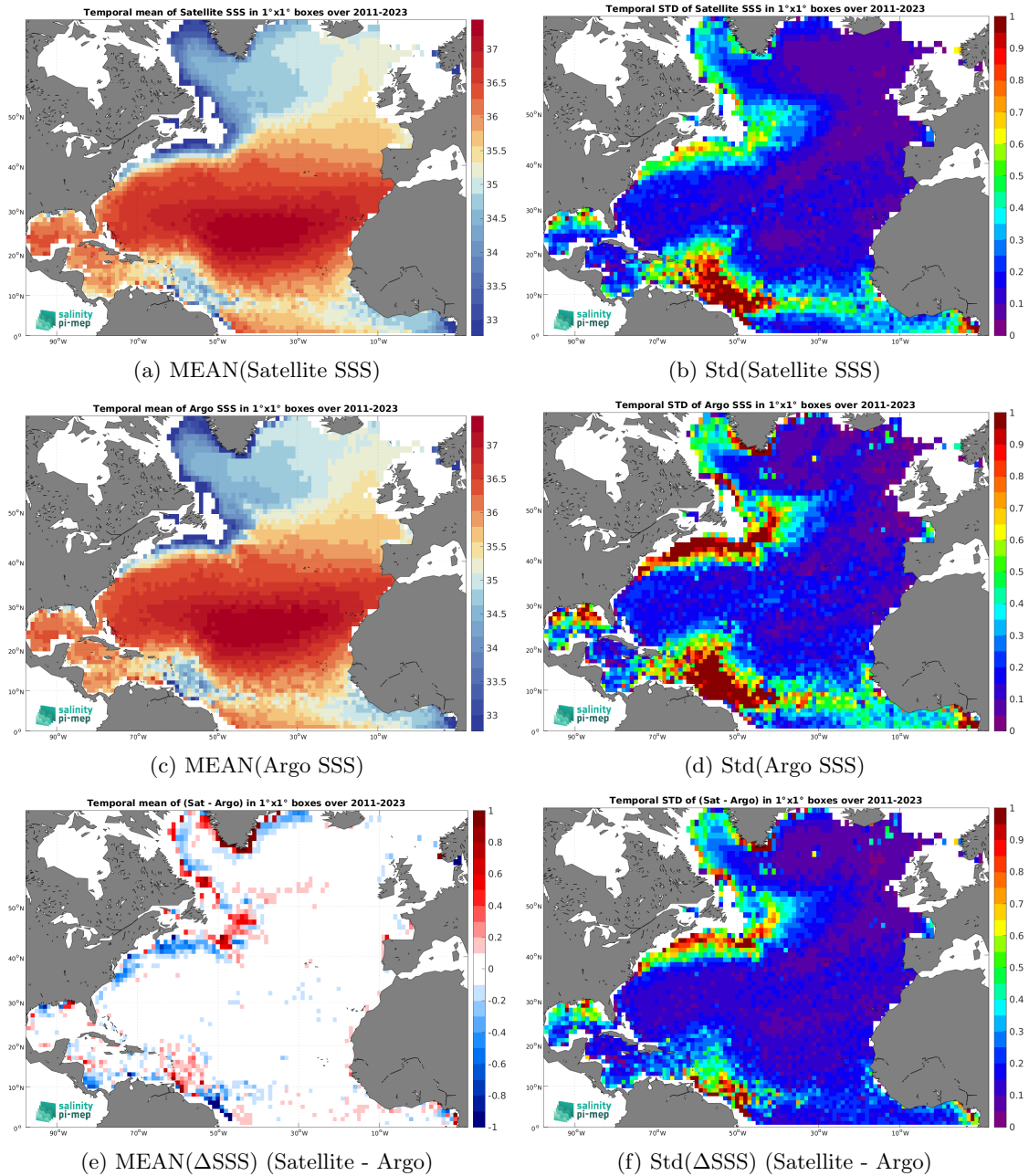
Figure 7: Temporal mean (left) and Std (right) of SSS from SMAP SSS L4 OI v3 - Daily (ESR) (top), Argo (middle), and of \Delta SSS (Satellite - Argo). Only match-up pairs are used to generate these maps.
