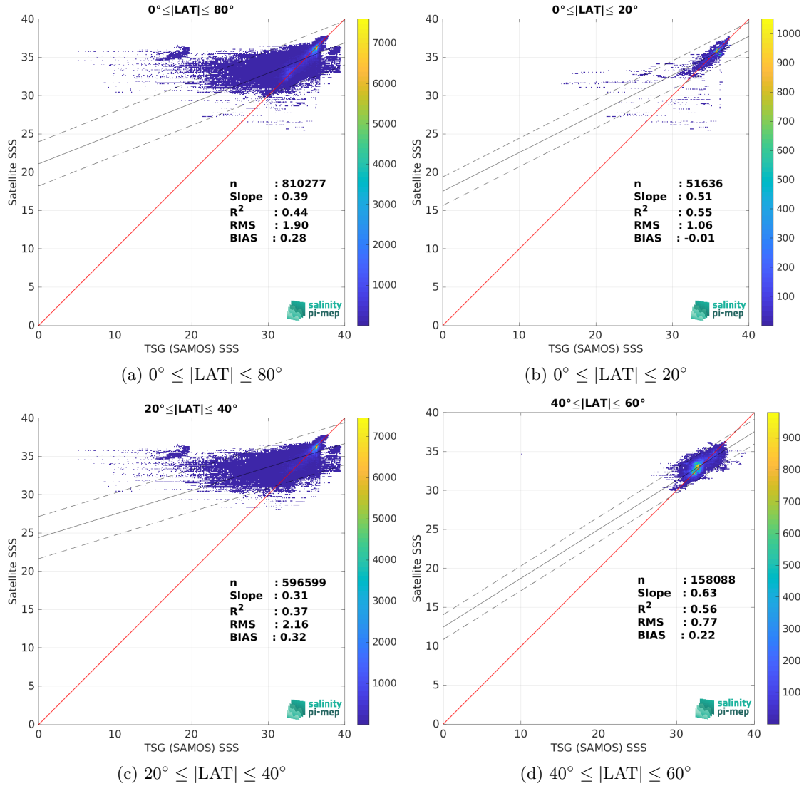
Figure 9: Contour maps of the concentration of SMAP SSS L4 OI v2 - 7 Days (ESR) SSS (y-axis) versus TSG (SAMOS) SSS (x-axis) at match-up pairs for different latitude bands. For each plot, the red line shows x=y . The black thin and dashed lines indicate a linear fit through the data cloud and the \pm 95\% confidence levels, respectively. The number match-up pairs n , the slope and R^2 coefficient of the linear fit, the root mean square (RMS) and the mean bias between satellite and in situ data are indicated for each latitude band in each plots.
