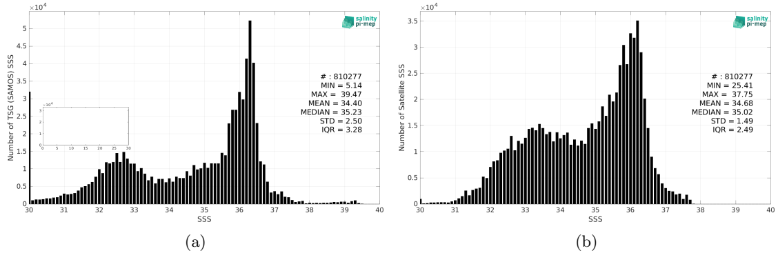
Figure 2: Histograms of SSS from TSG (SAMOS) (a) and SMAP SSS L4 OI v2 - 7 Days (ESR) (b) considering all match-up pairs per bins of 0.1 over the North Atlantic Ocean Pi-MEP region and for the full satellite product period.
