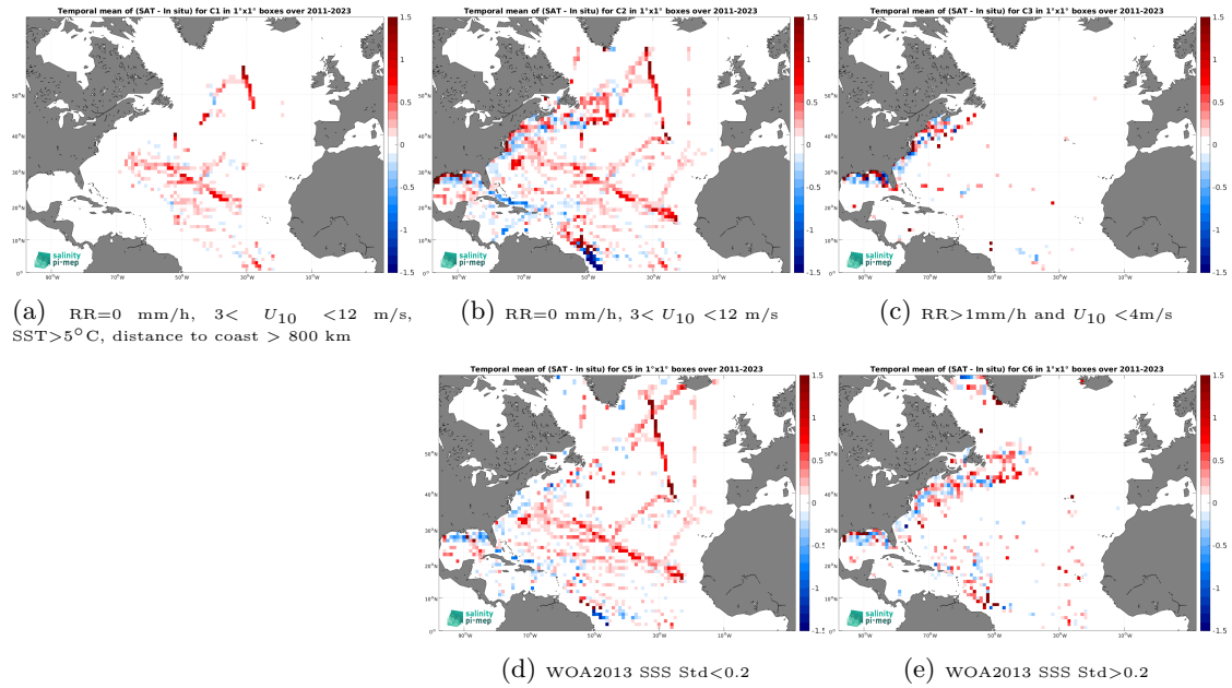
Figure 12: Temporal mean gridded over spatial boxes of size 1^\circ \times 1^\circ of \Delta\text{SSS} (SMAP SSS L4 OI v2 - 7 Days (ESR) - TSG (SAMOS)) for 5 different subdatasets corresponding to:RR=0 mm/h, 3 < U_{10} < 12 m/s, SST >5^\circ\text{C} , distance to coast > 800 km (a), RR=0 mm/h, 3 < U_{10} < 12 m/s (b), RR >1 mm/h and U_{10} < 4 m/s (c), WOA2013 SSS Std <0.2 (d), WOA2013 SSS Std >0.2 (e).
