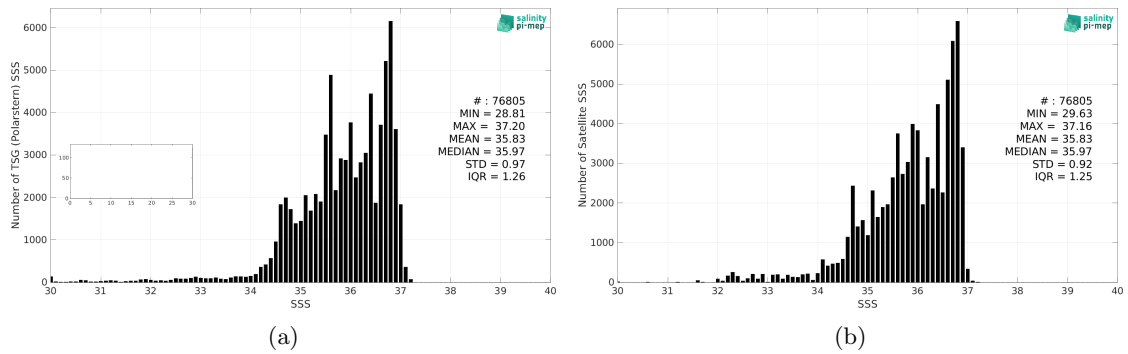
Figure 2: Histograms of SSS from TSG (Polarstern) (a) and SMAP SSS L4 OI v2 - 7 Days (ESR) (b) considering all match-up pairs per bins of 0.1 over the North Atlantic Ocean Pi-MEP region and for the full satellite product period.
