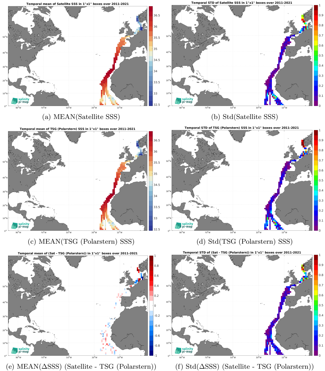
Figure 6: Temporal mean (left) and Std (right) of SSS from SMAP SSS L4 OI v2 - 7 Days (ESR) (top), TSG (Polarstern) (middle), and of \Delta SSS (Satellite - TSG (Polarstern)). Only match-up pairs are used to generate these maps.
