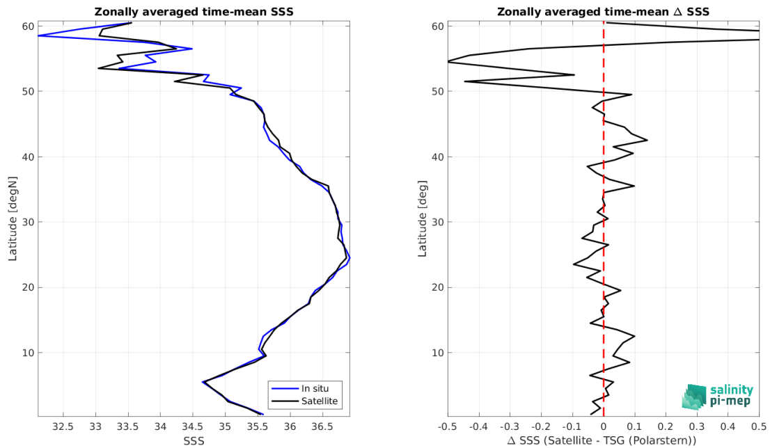
Figure 8: Left panel: Zonal mean SSS from SMAP SSS L4 OI v2 - 7 Days (ESR) satellite product (black) and from TSG (Polarstern) (blue). Right panel: Zonal mean of \Delta SSS (Satellite - TSG (Polarstern)) for all the collected Pi-MEP match-up pairs estimated over the full satellite product period.
