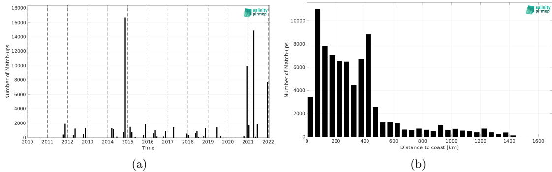
Figure 1: Number of match-ups between TSG (Polarstern) and SMAP SSS L4 OI v2 - 7 Days (ESR) SSS as a function of time (a) and as function of the distance to coast (b) over the North Atlantic Ocean Pi-MEP region and for the full satellite product period.
