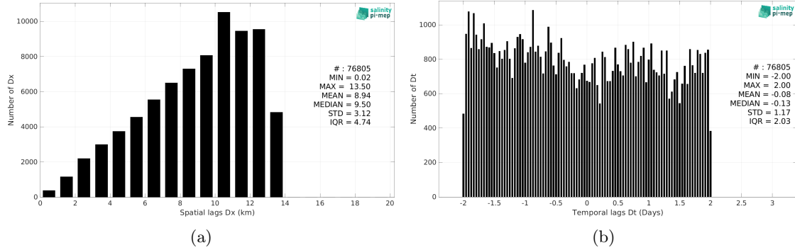
Figure 5: Histograms of the spatial (a) and temporal (b) lags between the location/time of the TSG (Polarstern) measurement and the date of the corresponding SMAP SSS L4 OI v2 - 7 Days (ESR) SSS pixel.
