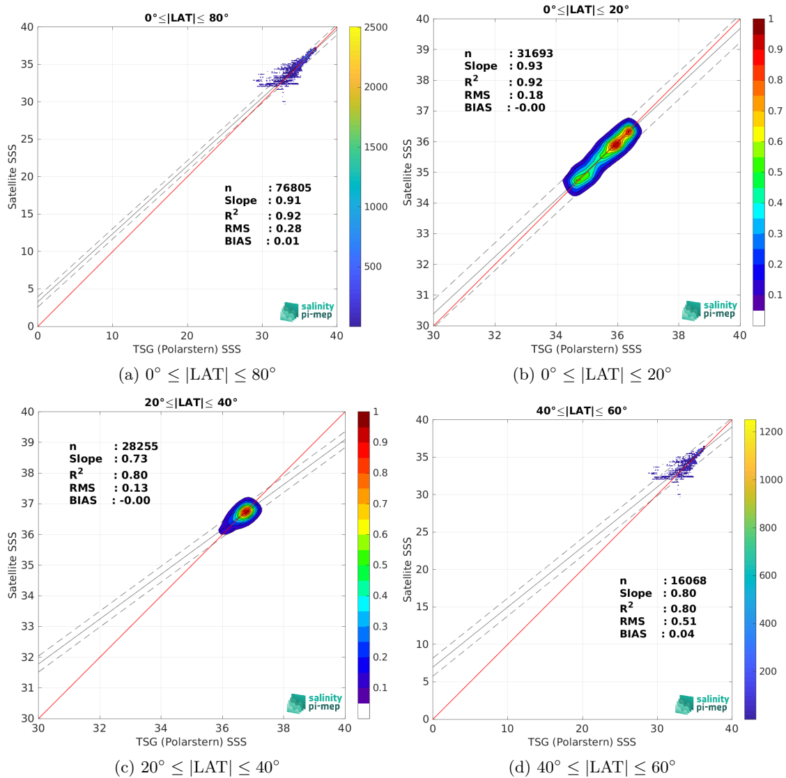
Figure 9: Contour maps of the concentration of SMAP SSS L4 OI v2 - 7 Days (ESR) SSS (y-axis) versus TSG (Polarstern) SSS (x-axis) at match-up pairs for different latitude bands. For each plot, the red line shows x=y . The black thin and dashed lines indicate a linear fit through the data cloud and the \pm 95\% confidence levels, respectively. The number match-up pairs n , the slope and R^2 coefficient of the linear fit, the root mean square (RMS) and the mean bias between satellite and in situ data are indicated for each latitude band in each plots.
