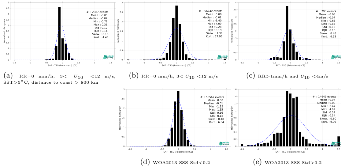
Figure 13: Normalized histogram of \Delta SSS (SMAP SSS L4 OI v2 - 7 Days (ESR) - TSG (Polarstern)) for 5 different subdatasets corresponding to: RR=0 mm/h, 3 < U_{10} < 12 m/s, SST>5°C, distance to coast > 800 km (a), RR=0 mm/h, 3 < U_{10} < 12 m/s (b), RR>1mm/h and U_{10} < 4 m/s (c), WOA2013 SSS Std<0.2 (d), WOA2013 SSS Std>0.2 (e).
