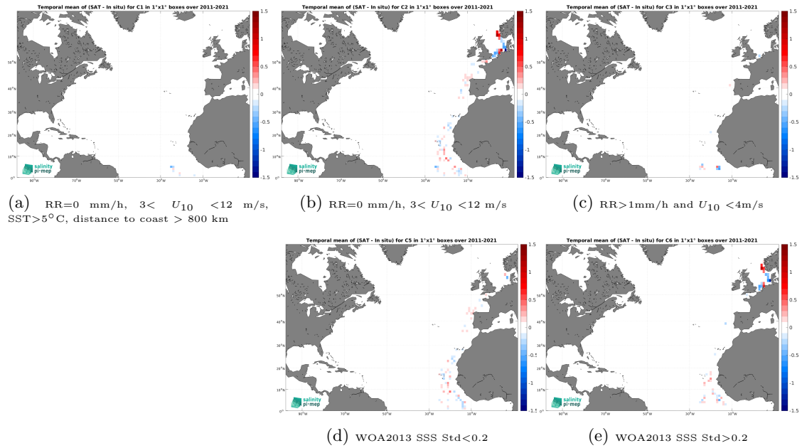
Figure 12: Temporal mean gridded over spatial boxes of size 1^\circ \times 1^\circ of \Delta\text{SSS} (SMAP SSS L4 OI v2 - 7 Days (ESR) - TSG (Polarstern)) for 5 different subdatasets corresponding to:RR=0 mm/h, 3 < U_{10} < 12 m/s, SST >5^\circ\text{C} , distance to coast > 800 km (a), RR=0 mm/h, 3 < U_{10} < 12 m/s (b), RR >1 mm/h and U_{10} < 4 m/s (c), WOA2013 SSS Std <0.2 (d), WOA2013 SSS Std >0.2 (e).
