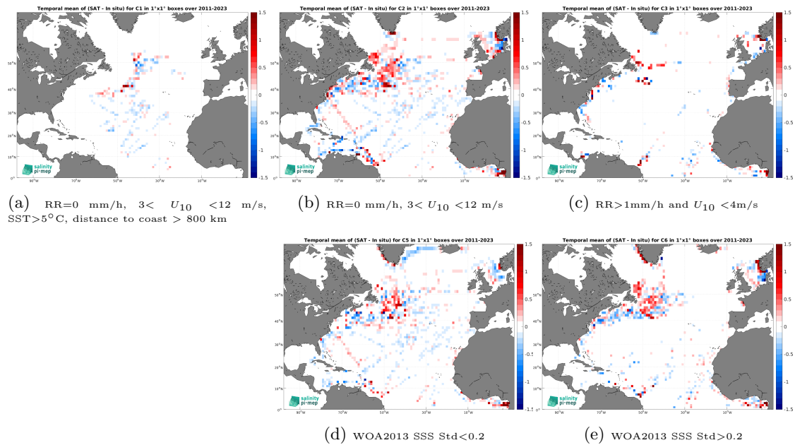
Figure 12: Temporal mean gridded over spatial boxes of size 1^\circ \times 1^\circ of \Delta\text{SSS} (SMAP SSS L4 OI v2 - 7 Days (ESR) - TSG (LEGOS-DM)) for 5 different subdatasets corresponding to:RR=0 mm/h, 3 < U_{10} < 12 m/s, SST >5^\circ\text{C} , distance to coast > 800 km (a), RR=0 mm/h, 3 < U_{10} < 12 m/s (b), RR >1 mm/h and U_{10} < 4 m/s (c), WOA2013 SSS Std <0.2 (d), WOA2013 SSS Std >0.2 (e).
