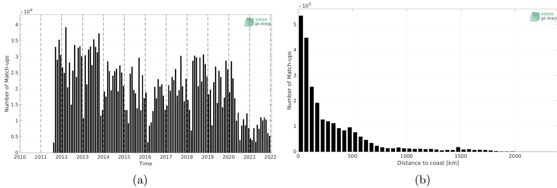
Figure 1: Number of match-ups between TSG (LEGOS-DM) and SMAP SSS L4 OI v2 - 7 Days (ESR) SSS as a function of time (a) and as function of the distance to coast (b) over the North Atlantic Ocean Pi-MEP region and for the full satellite product period.
