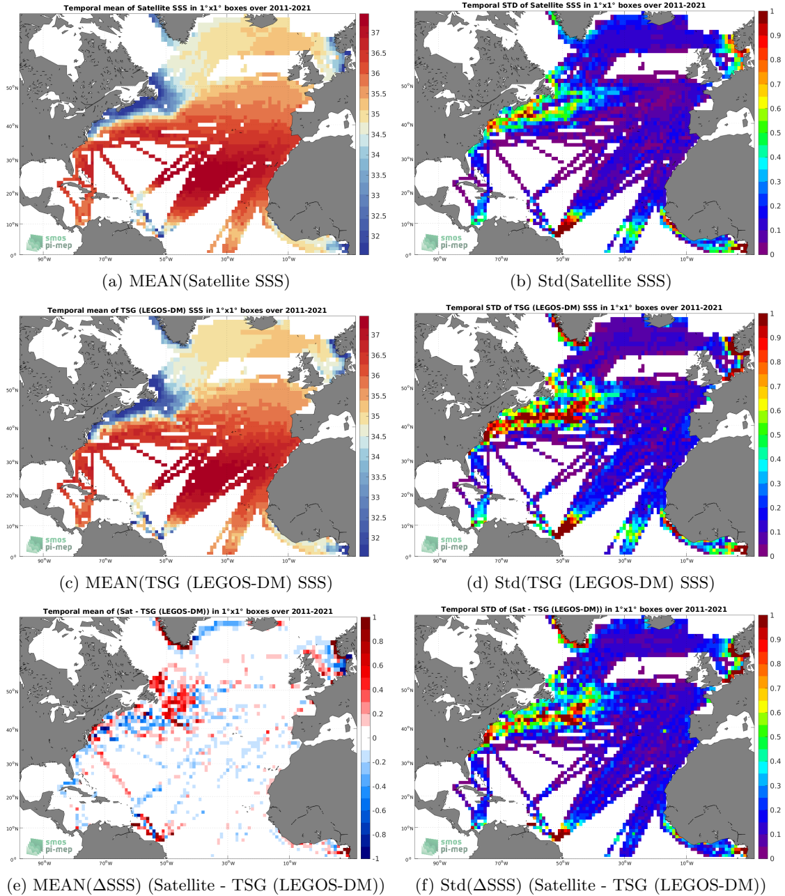
Figure 6: Temporal mean (left) and Std (right) of SSS from SMAP SSS L4 OI v2 - 7 Days (ESR) (top), TSG (LEGOS-DM) (middle), and of \Delta SSS (Satellite - TSG (LEGOS-DM)). Only match-up pairs are used to generate these maps.
