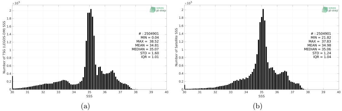
Figure 2: Histograms of SSS from TSG (LEGOS-DM) (a) and SMAP SSS L4 OI v2 - 7 Days (ESR) (b) considering all match-up pairs per bins of 0.1 over the North Atlantic Ocean Pi-MEP region and for the full satellite product period.
