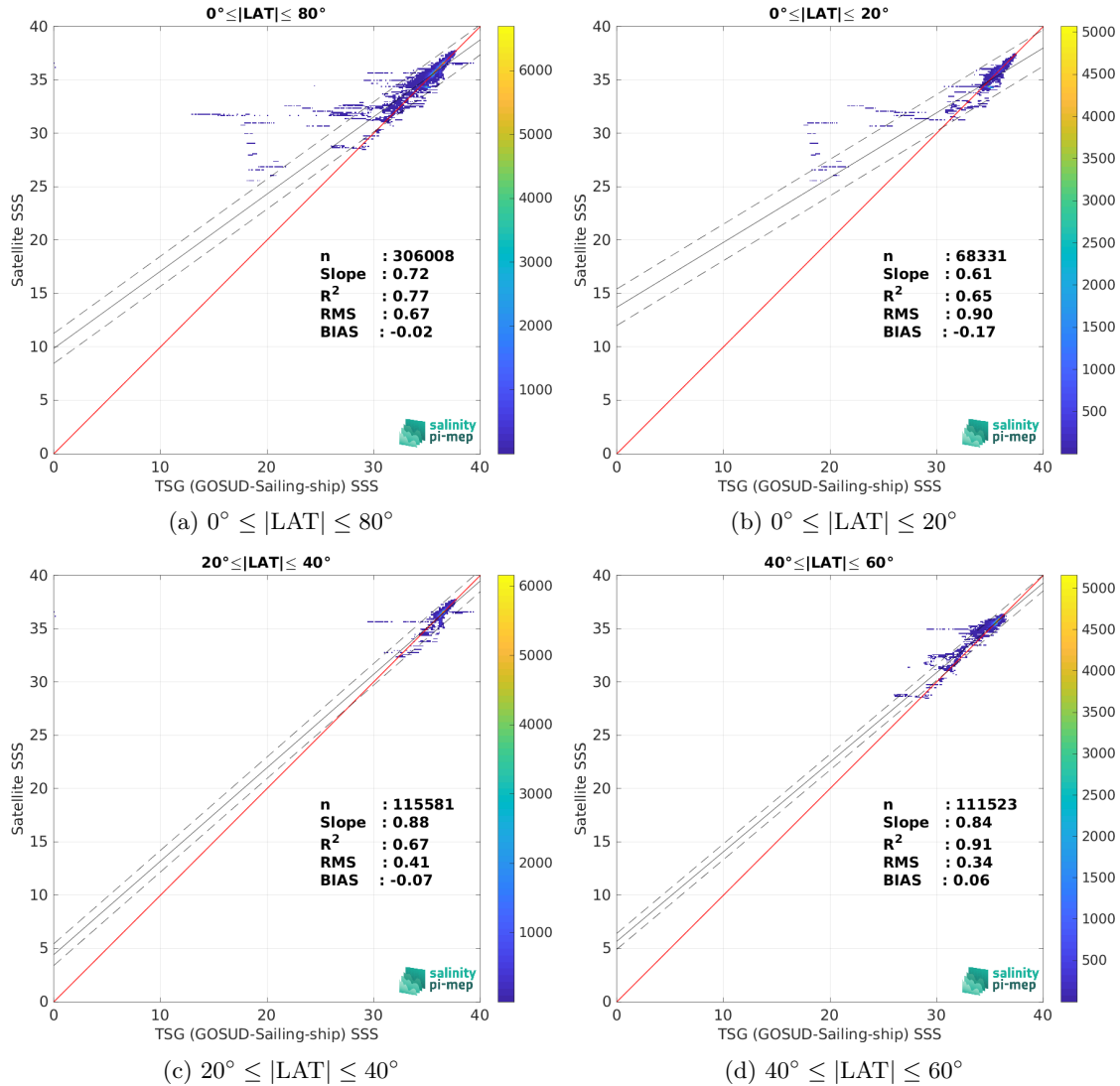
Figure 9: Contour maps of the concentration of SMAP SSS L4 OI v2 - 7 Days (ESR) SSS (y-axis) versus TSG (GOSUD-Sailing-ship) SSS (x-axis) at match-up pairs for different latitude bands. For each plot, the red line shows x=y . The black thin and dashed lines indicate a linear fit through the data cloud and the \pm 95\% confidence levels, respectively. The number match-up pairs n , the slope and R^2 coefficient of the linear fit, the root mean square (RMS) and the mean bias between satellite and in situ data are indicated for each latitude band in each plots.
