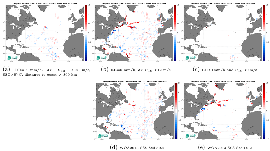
Figure 12: Temporal mean gridded over spatial boxes of size 1^\circ \times 1^\circ of \Delta\text{SSS} (SMAP SSS L4 OI v2 - 7 Days (ESR) - TSG (GOSUD-Sailing-ship)) for 5 different subdatasets corresponding to:RR=0 mm/h, 3 < U_{10} < 12 m/s, SST > 5°C, distance to coast > 800 km (a), RR=0 mm/h, 3 < U_{10} < 12 m/s (b), RR > 1mm/h and U_{10} < 4 m/s (c), WOA2013 SSS Std < 0.2 (d), WOA2013 SSS Std > 0.2 (e).
