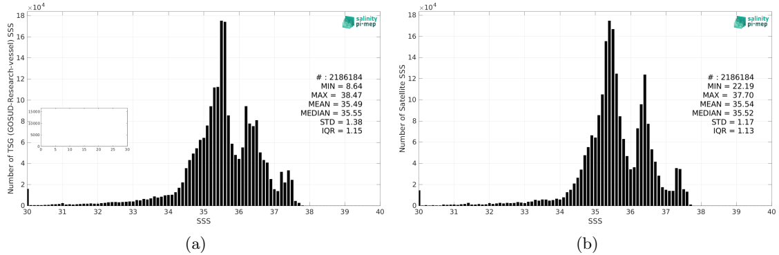
Figure 2: Histograms of SSS from TSG (GOSUD-Research-vessel) (a) and SMAP SSS L4 OI v2 - 7 Days (ESR) (b) considering all match-up pairs per bins of 0.1 over the North Atlantic Ocean Pi-MEP region and for the full satellite product period.
