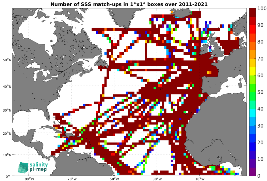
Figure 4: Number of SSS match-ups between TSG (GOSUD-Research-vessel) SSS and the SMAP SSS L4 OI v2 - 7 Days (ESR) SSS product for the North Atlantic Ocean Pi-MEP region over 1^\circ \times 1^\circ boxes and for the full satellite product period.
