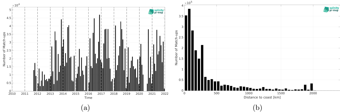
Figure 1: Number of match-ups between TSG (GOSUD-Research-vessel) and SMAP SSS L4 OI v2 - 7 Days (ESR) SSS as a function of time (a) and as function of the distance to coast (b) over the North Atlantic Ocean Pi-MEP region and for the full satellite product period.
