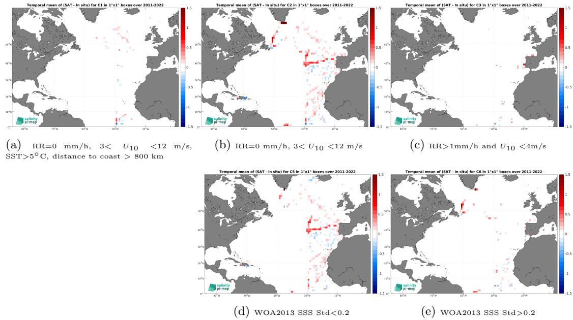
Figure 12: Temporal mean gridded over spatial boxes of size 1^\circ \times 1^\circ of \Delta\text{SSS} (SMAP SSS L4 OI v2 - 7 Days (ESR) - TSG (CSIC-UTM)) for 5 different subdatasets corresponding to:RR=0 mm/h, 3 < U_{10} < 12 m/s, SST > 5^\circ\text{C} , distance to coast > 800 km (a), RR=0 mm/h, 3 < U_{10} < 12 m/s (b), RR > 1 mm/h and U_{10} < 4 m/s (c), WOA2013 SSS Std < 0.2 (d), WOA2013 SSS Std > 0.2 (e).
