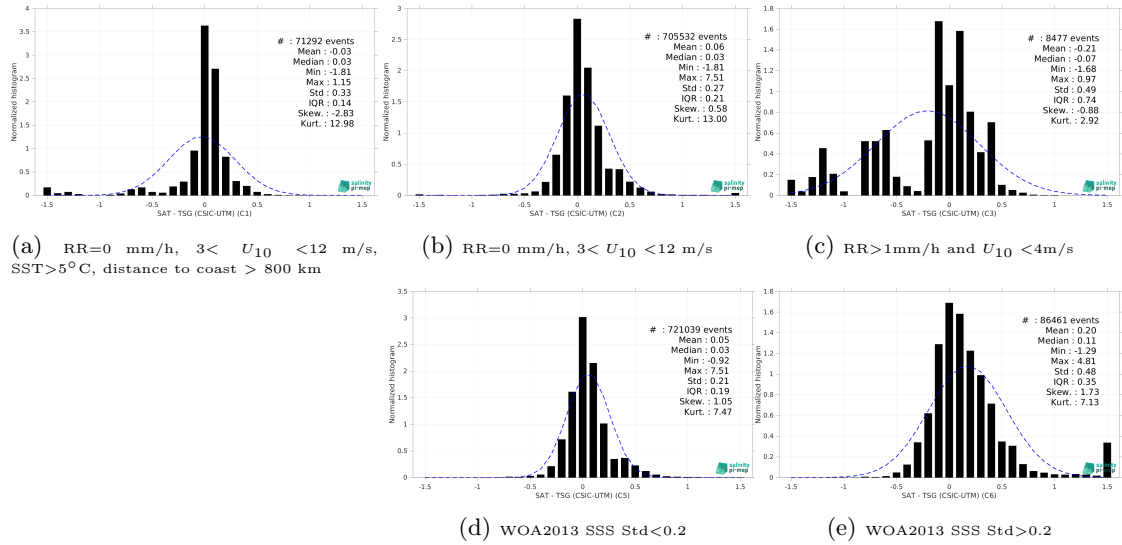
Figure 13: Normalized histogram of \Delta\text{SSS} (SMAP SSS L4 OI v2 - 7 Days (ESR) - TSG (CSIC-UTM)) for 5 different subdatasets corresponding to: RR=0 mm/h, 3 < U_{10} < 12 m/s, SST>5°C, distance to coast > 800 km (a), RR=0 mm/h, 3 < U_{10} < 12 m/s (b), RR>1mm/h and U_{10} < 4 m/s (c), WOA2013 SSS Std<0.2 (d), WOA2013 SSS Std>0.2 (e).
