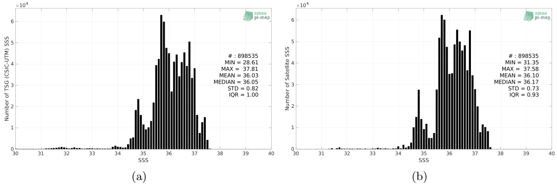
Figure 2: Histograms of SSS from TSG (CSIC-UTM) (a) and SMAP SSS L4 OI v2 - 7 Days (ESR) (b) considering all match-up pairs per bins of 0.1 over the North Atlantic Ocean Pi-MEP region and for the full satellite product period.
