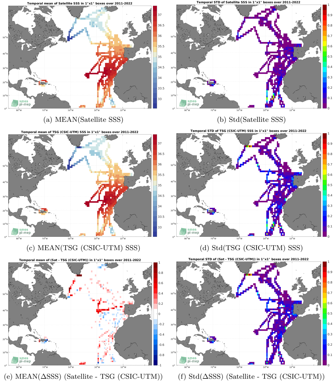
Figure 6: Temporal mean (left) and Std (right) of SSS from SMAP SSS L4 OI v2 - 7 Days (ESR) (top), TSG (CSIC-UTM) (middle), and of \Delta SSS (Satellite - TSG (CSIC-UTM)). Only match-up pairs are used to generate these maps.
