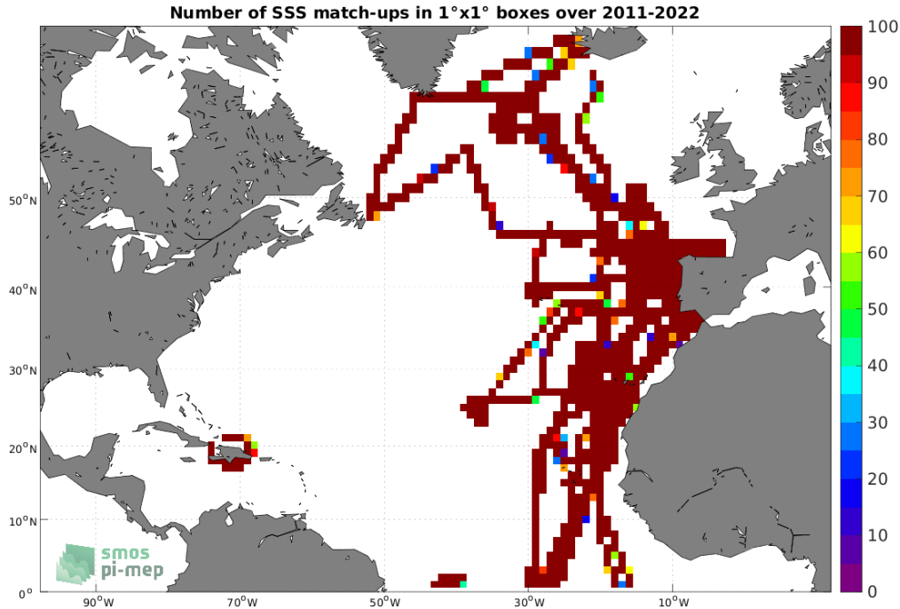
Figure 4: Number of SSS match-ups between TSG (CSIC-UTM) SSS and the SMAP SSS L4 OI v2 - 7 Days (ESR) SSS product for the North Atlantic Ocean Pi-MEP region over 1^\circ \times 1^\circ boxes and for the full satellite product period.
