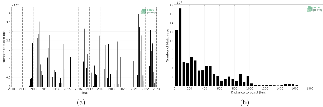
Figure 1: Number of match-ups between TSG (CSIC-UTM) and SMAP SSS L4 OI v2 - 7 Days (ESR) SSS as a function of time (a) and as function of the distance to coast (b) over the North Atlantic Ocean Pi-MEP region and for the full satellite product period.
