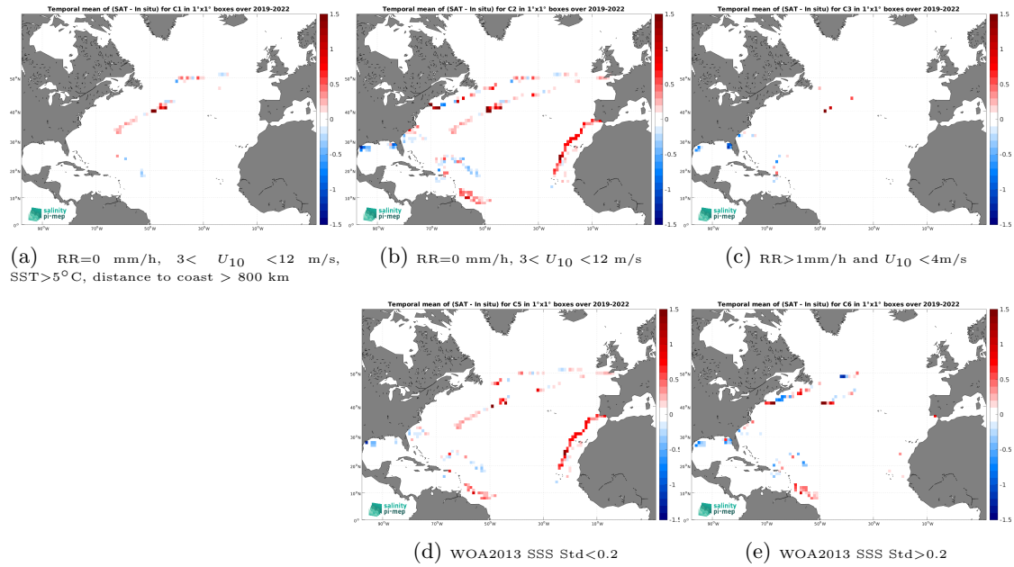
Figure 12: Temporal mean gridded over spatial boxes of size 1^\circ \times 1^\circ of \Delta\text{SSS} (SMAP SSS L4 OI v2 - 7 Days (ESR) - Saildrone) for 5 different subdatasets corresponding to:RR=0 mm/h, 3 < U_{10} < 12 m/s, SST >5^\circ\text{C} , distance to coast > 800 km (a), RR=0 mm/h, 3 < U_{10} < 12 m/s (b), RR >1 mm/h and U_{10} < 4 m/s (c), WOA2013 SSS Std <0.2 (d), WOA2013 SSS Std >0.2 (e).
