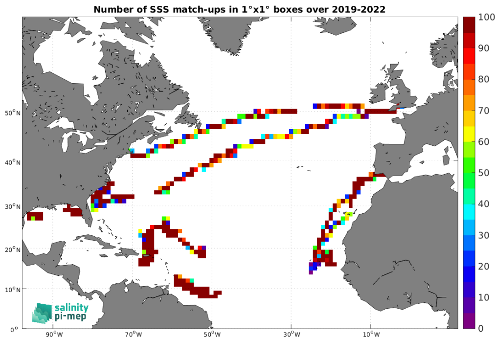
Figure 4: Number of SSS match-ups between Saildrone SSS and the SMAP SSS L4 OI v2 - 7 Days (ESR) SSS product for the North Atlantic Ocean Pi-MEP region over 1^\circ \times 1^\circ boxes and for the full satellite product period.
