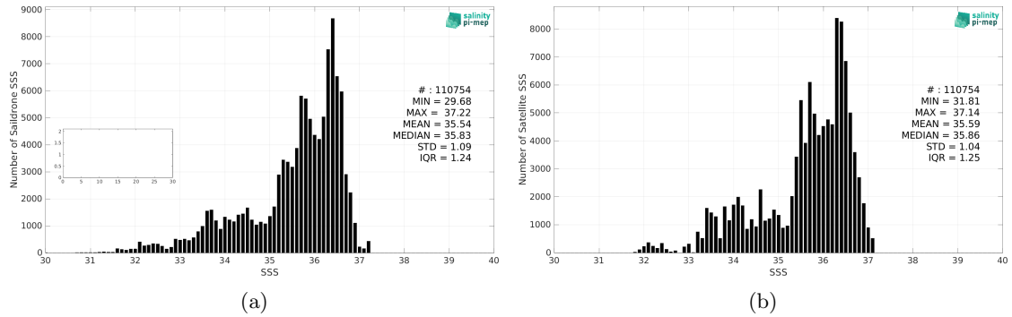
Figure 2: Histograms of SSS from Saildrone (a) and SMAP SSS L4 OI v2 - 7 Days (ESR) (b) considering all match-up pairs per bins of 0.1 over the North Atlantic Ocean Pi-MEP region and for the full satellite product period.
