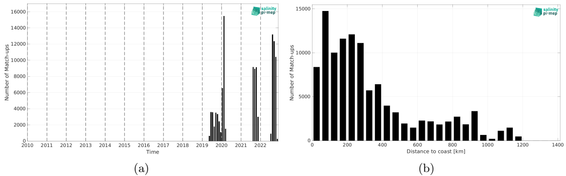
Figure 1: Number of match-ups between Saildrone and SMAP SSS L4 OI v2 - 7 Days (ESR) SSS as a function of time (a) and as function of the distance to coast (b) over the North Atlantic Ocean Pi-MEP region and for the full satellite product period.
