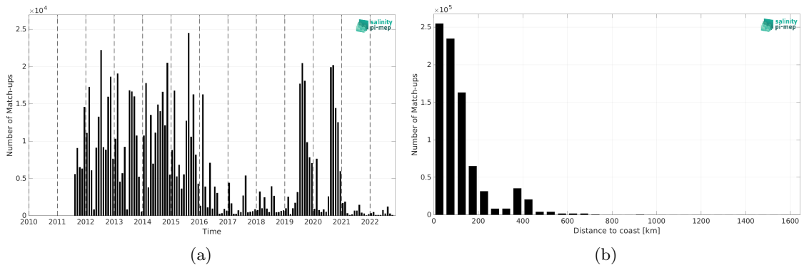
Figure 1: Number of match-ups between ICES and SMAP SSS L4 OI v2 - 7 Days (ESR) SSS as a function of time (a) and as function of the distance to coast (b) over the North Atlantic Ocean Pi-MEP region and for the full satellite product period.
