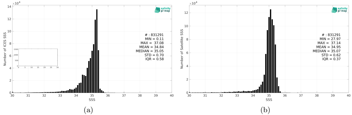
Figure 2: Histograms of SSS from ICES (a) and SMAP SSS L4 OI v2 - 7 Days (ESR) (b) considering all match-up pairs per bins of 0.1 over the North Atlantic Ocean Pi-MEP region and for the full satellite product period.
