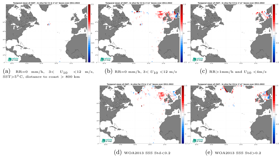
Figure 12: Temporal mean gridded over spatial boxes of size 1^\circ \times 1^\circ of \Delta\text{SSS} (SMAP SSS L4 OI v2 - 7 Days (ESR) - ICES) for 5 different subdatasets corresponding to:RR=0 mm/h, 3 < U_{10} < 12 m/s, SST >5^\circ\text{C} , distance to coast > 800 km (a), RR=0 mm/h, 3 < U_{10} < 12 m/s (b), RR >1 mm/h and U_{10} < 4 m/s (c), WOA2013 SSS Std <0.2 (d), WOA2013 SSS Std >0.2 (e).
