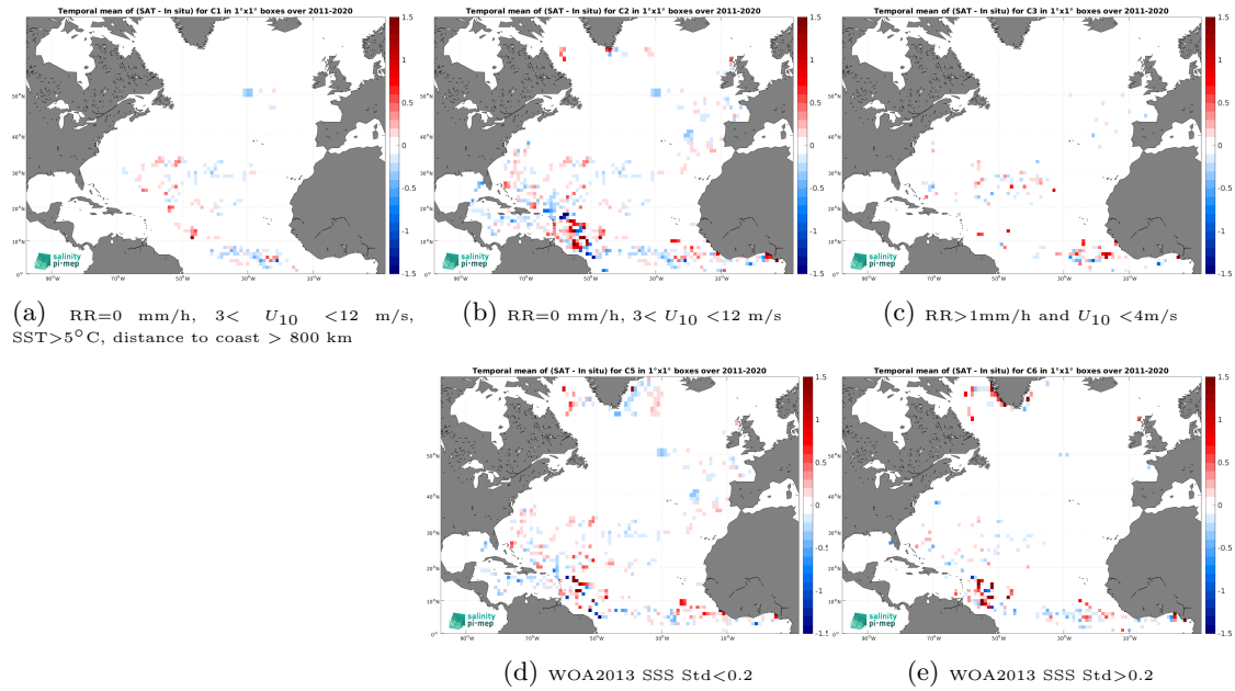
Figure 11: Temporal mean gridded over spatial boxes of size 1^\circ \times 1^\circ of \Delta\text{SSS} (SMAP SSS L4 OI v2 - 7 Days (ESR) - Surface drifters) for 5 different subdatasets corresponding to:RR=0 mm/h, 3 < U_{10} < 12 m/s, SST >5^\circ\text{C} , distance to coast > 800 km (a), RR=0 mm/h, 3 < U_{10} < 12 m/s (b), RR >1 mm/h and U_{10} < 4 m/s (c), WOA2013 SSS Std <0.2 (d), WOA2013 SSS Std >0.2 (e).
