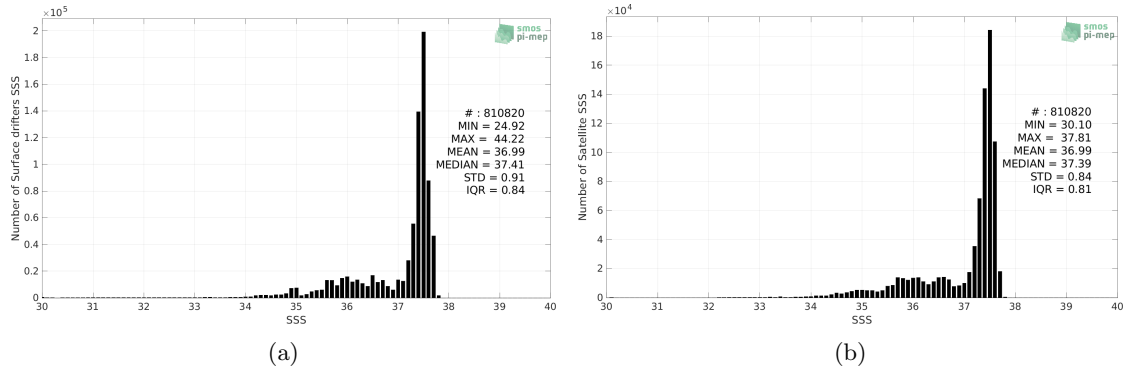
Figure 2: Histograms of SSS from Surface drifters (a) and SMAP SSS L4 OI v2 - 7 Days (ESR) (b) considering all match-up pairs per bins of 0.1 over the North Atlantic Ocean Pi-MEP region and for the full satellite product period.
