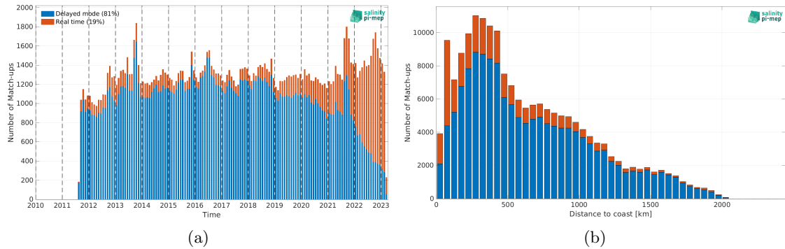
Figure 1: Number of match-ups between Argo and SMAP SSS L4 OI v2 - 7 Days (ESR) SSS as a function of time (a) and as function of the distance to coast (b) over the North Atlantic Ocean Pi-MEP region and for the full satellite product period.
