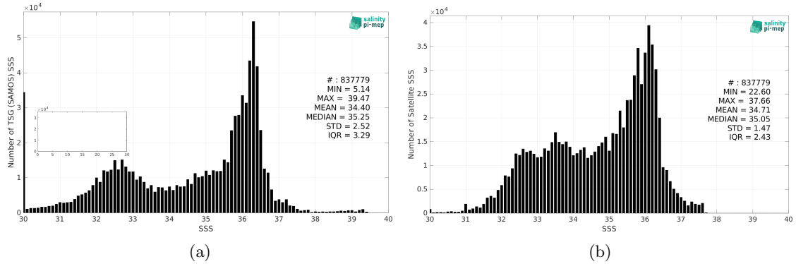
Figure 2: Histograms of SSS from TSG (SAMOS) (a) and SMAP SSS L4 OI v2 - Monthly (IPRC) (b) considering all match-up pairs per bins of 0.1 over the North Atlantic Ocean Pi-MEP region and for the full satellite product period.
