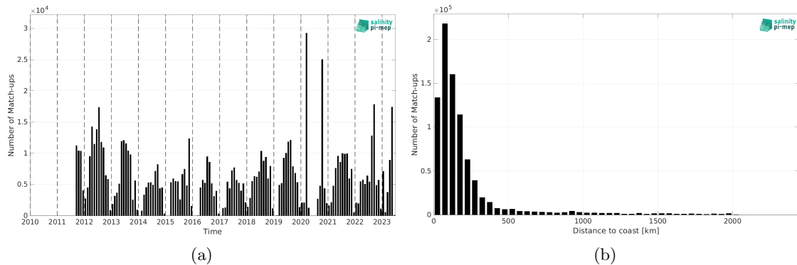
Figure 1: Number of match-ups between TSG (SAMOS) and SMAP SSS L4 OI v2 - Monthly (IPRC) SSS as a function of time (a) and as function of the distance to coast (b) over the North Atlantic Ocean Pi-MEP region and for the full satellite product period.
