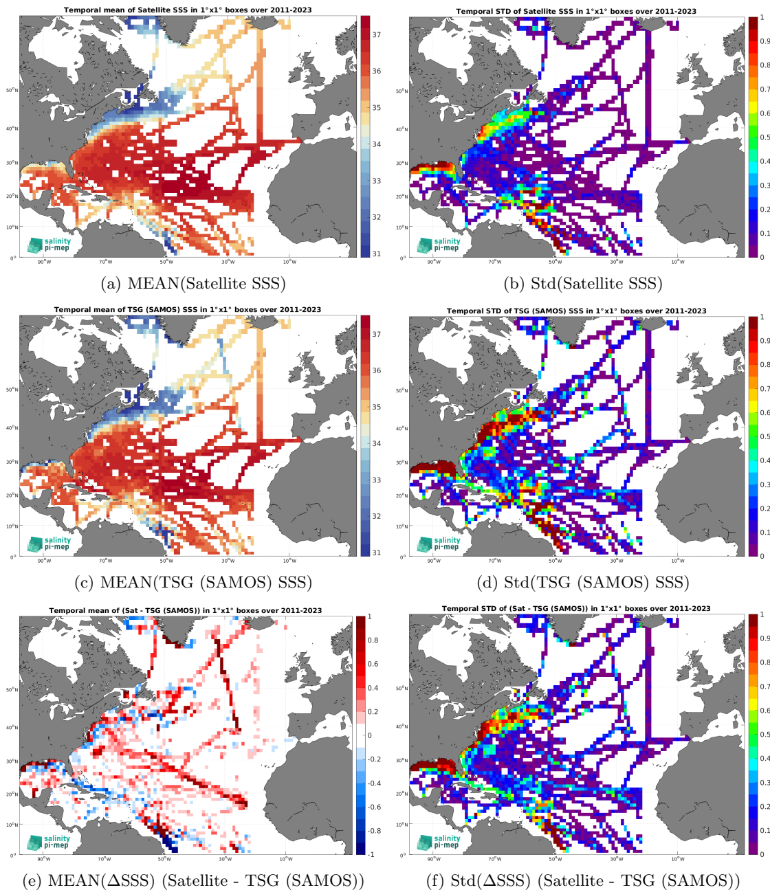
Figure 6: Temporal mean (left) and Std (right) of SSS from SMAP SSS L4 OI v2 - Monthly (IPRC) (top), TSG (SAMOS) (middle), and of \Delta SSS (Satellite - TSG (SAMOS)). Only match-up pairs are used to generate these maps.
