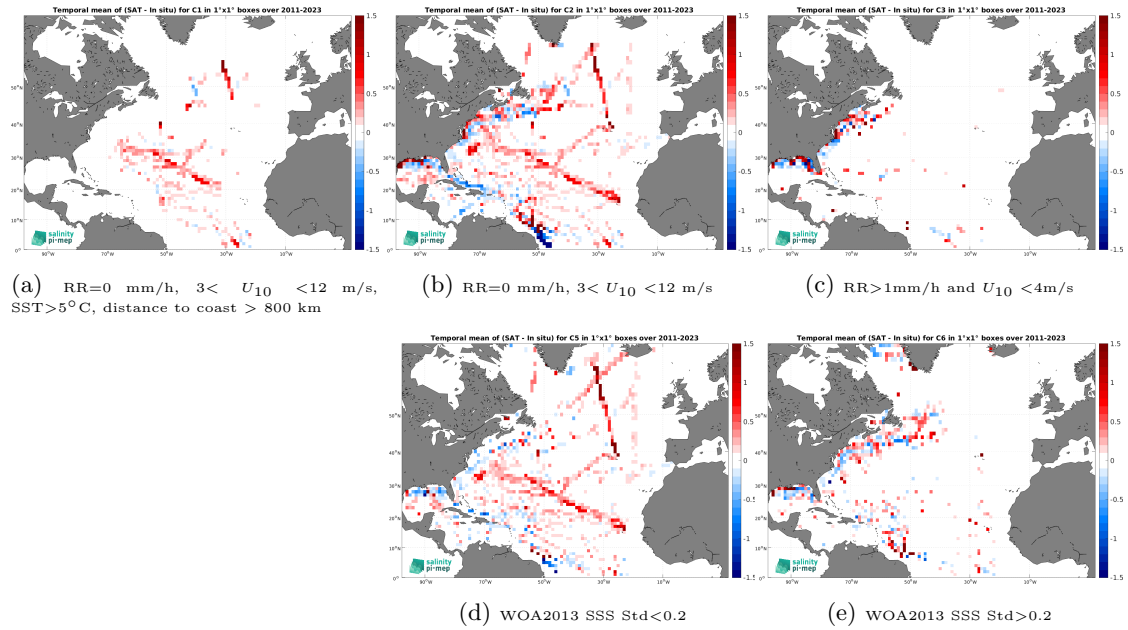
Figure 12: Temporal mean gridded over spatial boxes of size 1^\circ \times 1^\circ of \Delta\text{SSS} (SMAP SSS L4 OI v2 - Monthly (IPRC) - TSG (SAMOS)) for 5 different subdatasets corresponding to:RR=0 mm/h, 3 < U_{10} < 12 m/s, SST >5^\circ\text{C} , distance to coast > 800 km (a), RR=0 mm/h, 3 < U_{10} < 12 m/s (b), RR >1 mm/h and U_{10} < 4 m/s (c), WOA2013 SSS Std <0.2 (d), WOA2013 SSS Std >0.2 (e).
