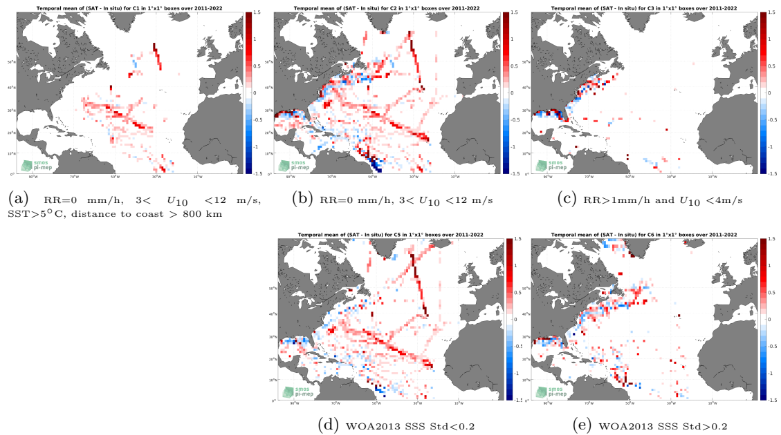
Figure 12: Temporal mean gridded over spatial boxes of size 1^\circ \times 1^\circ of \Delta SSS (SMAP SSS L4 OI v2 - Monthly (IPRC) - TSG (SAMOS)) for 5 different subdatasets corresponding to:RR=0 mm/h, 3 < U_{10} < 12 m/s, SST >5^\circ\text{C} , distance to coast > 800 km (a), RR=0 mm/h, 3 < U_{10} < 12 m/s (b), RR >1 mm/h and U_{10} < 4 m/s (c), WOA2013 SSS Std <0.2 (d), WOA2013 SSS Std >0.2 (e).
