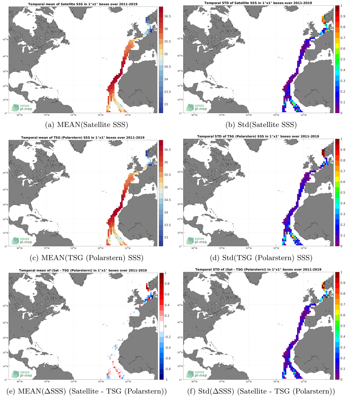
Figure 6: Temporal mean (left) and Std (right) of SSS from SMAP SSS L4 OI v2 - Monthly (IPRC) (top), TSG (Polarstern) (middle), and of \Delta SSS (Satellite - TSG (Polarstern)). Only match-up pairs are used to generate these maps.
