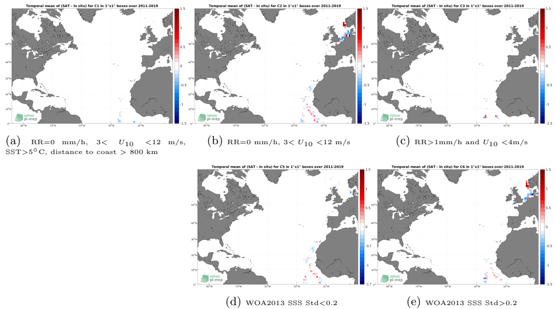
Figure 12: Temporal mean gridded over spatial boxes of size 1^\circ \times 1^\circ of \Delta SSS (SMAP SSS L4 OI v2 - Monthly (IPRC) - TSG (Polarstern)) for 5 different subdatasets corresponding to:RR=0 mm/h, 3 < U_{10} < 12 m/s, SST >5^\circ\text{C} , distance to coast > 800 km (a), RR=0 mm/h, 3 < U_{10} < 12 m/s (b), RR >1 mm/h and U_{10} < 4 m/s (c), WOA2013 SSS Std <0.2 (d), WOA2013 SSS Std >0.2 (e).
