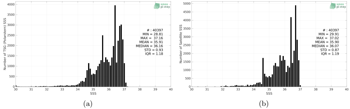
Figure 2: Histograms of SSS from TSG (Polarstern) (a) and SMAP SSS L4 OI v2 - Monthly (IPRC) (b) considering all match-up pairs per bins of 0.1 over the North Atlantic Ocean Pi-MEP region and for the full satellite product period.
