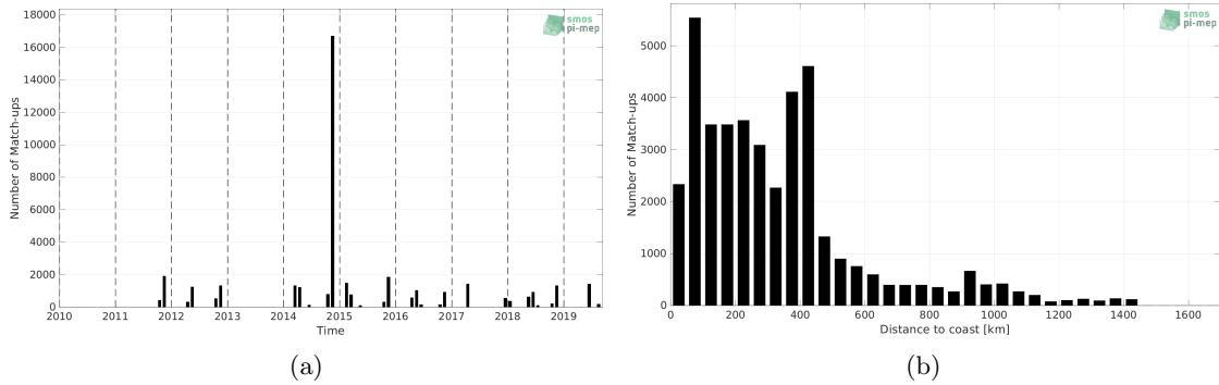
Figure 1: Number of match-ups between TSG (Polarstern) and SMAP SSS L4 OI v2 - Monthly (IPRC) SSS as a function of time (a) and as function of the distance to coast (b) over the North Atlantic Ocean Pi-MEP region and for the full satellite product period.
