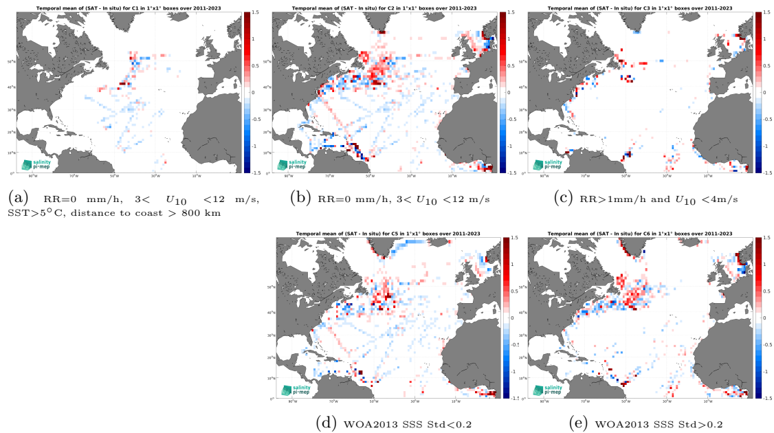
Figure 12: Temporal mean gridded over spatial boxes of size 1^\circ \times 1^\circ of \Delta\text{SSS} (SMAP SSS L4 OI v2 - Monthly (IPRC) - TSG (LEGOS-DM)) for 5 different subdatasets corresponding to:RR=0 mm/h, 3 < U_{10} < 12 m/s, SST > 5^\circ\text{C} , distance to coast > 800 km (a), RR=0 mm/h, 3 < U_{10} < 12 m/s (b), RR > 1 mm/h and U_{10} < 4 m/s (c), WOA2013 SSS Std < 0.2 (d), WOA2013 SSS Std > 0.2 (e).
