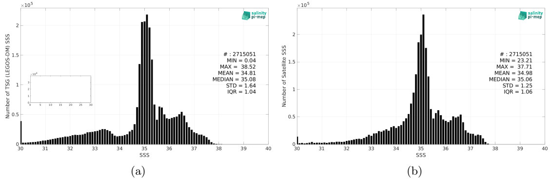
Figure 2: Histograms of SSS from TSG (LEGOS-DM) (a) and SMAP SSS L4 OI v2 - Monthly (IPRC) (b) considering all match-up pairs per bins of 0.1 over the North Atlantic Ocean Pi-MEP region and for the full satellite product period.
