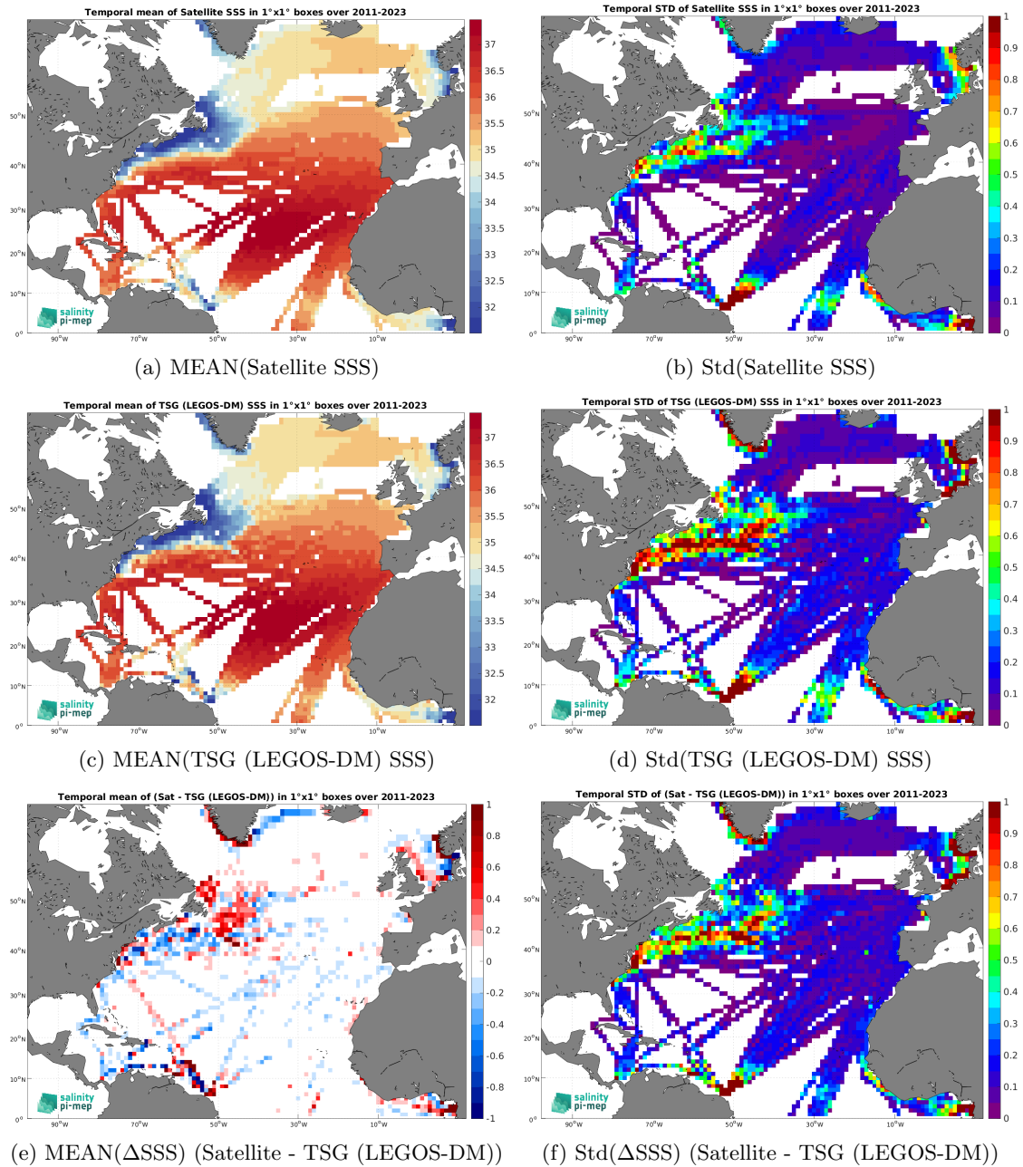
Figure 6: Temporal mean (left) and Std (right) of SSS from SMAP SSS L4 OI v2 - Monthly (IPRC) (top), TSG (LEGOS-DM) (middle), and of \Delta SSS (Satellite - TSG (LEGOS-DM)). Only match-up pairs are used to generate these maps.
