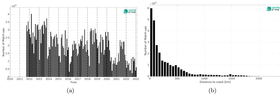
Figure 1: Number of match-ups between TSG (LEGOS-DM) and SMAP SSS L4 OI v2 - Monthly (IPRC) SSS as a function of time (a) and as function of the distance to coast (b) over the North Atlantic Ocean Pi-MEP region and for the full satellite product period.
