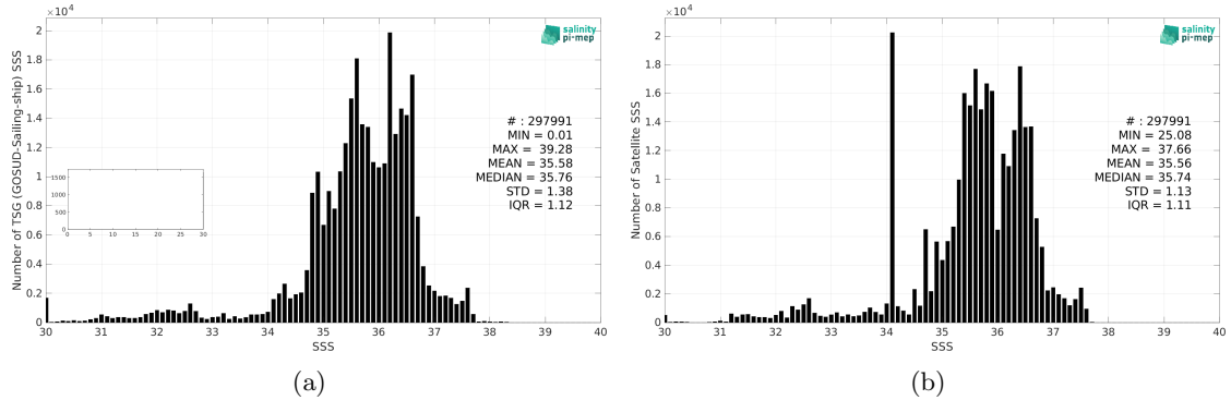
Figure 2: Histograms of SSS from TSG (GOSUD-Sailing-ship) (a) and SMAP SSS L4 OI v2 - Monthly (IPRC) (b) considering all match-up pairs per bins of 0.1 over the North Atlantic Ocean Pi-MEP region and for the full satellite product period.
