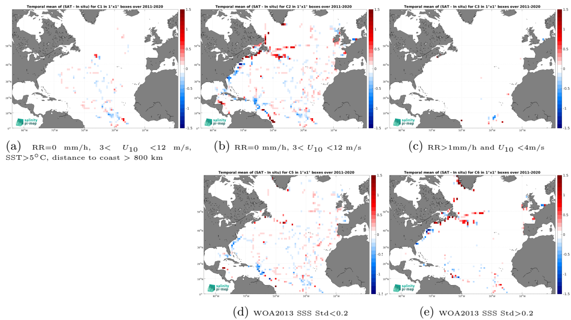
Figure 12: Temporal mean gridded over spatial boxes of size 1^\circ \times 1^\circ of \Delta\text{SSS} (SMAP SSS L4 OI v2 - Monthly (IPRC) - TSG (GOSUD-Sailing-ship)) for 5 different subdatasets corresponding to:RR=0 mm/h, 3 < U_{10} < 12 m/s, SST > 5°C, distance to coast > 800 km (a), RR=0 mm/h, 3 < U_{10} < 12 m/s (b), RR > 1mm/h and U_{10} < 4 m/s (c), WOA2013 SSS Std < 0.2 (d), WOA2013 SSS Std > 0.2 (e).
