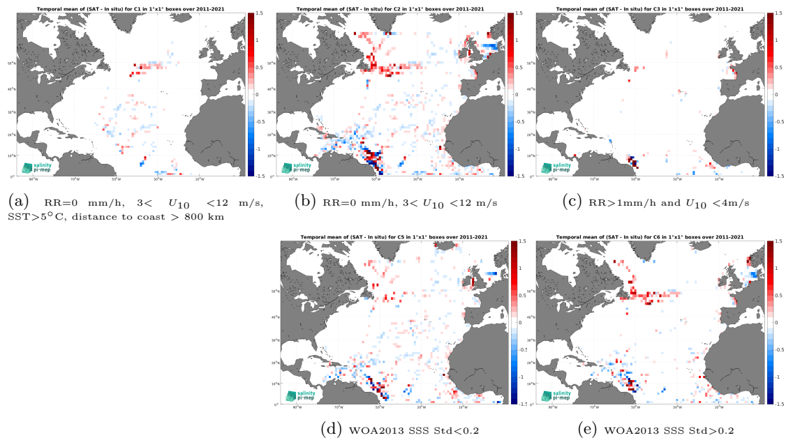
Figure 12: Temporal mean gridded over spatial boxes of size 1^\circ \times 1^\circ of \Delta\text{SSS} (SMAP SSS L4 OI v2 - Monthly (IPRC) - TSG (GOSUD-Research-vessel)) for 5 different subdatasets corresponding to:RR=0 mm/h, 3 < U_{10} < 12 m/s, SST>5°C, distance to coast > 800 km (a), RR=0 mm/h, 3 < U_{10} < 12 m/s (b), RR>1mm/h and U_{10} < 4 m/s (c), WOA2013 SSS Std<0.2 (d), WOA2013 SSS Std>0.2 (e).
