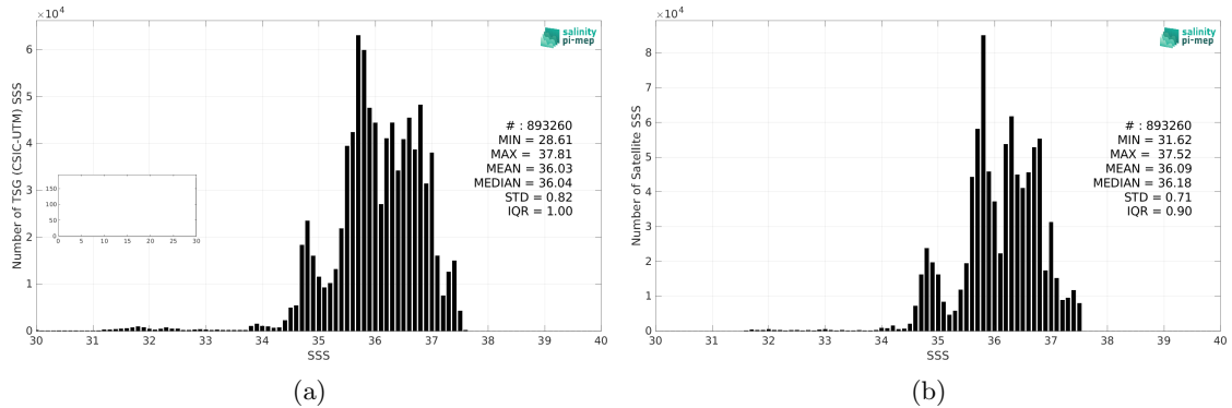
Figure 2: Histograms of SSS from TSG (CSIC-UTM) (a) and SMAP SSS L4 OI v2 - Monthly (IPRC) (b) considering all match-up pairs per bins of 0.1 over the North Atlantic Ocean Pi-MEP region and for the full satellite product period.
