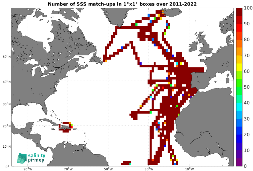
Figure 4: Number of SSS match-ups between TSG (CSIC-UTM) SSS and the SMAP SSS L4 OI v2 - Monthly (IPRC) SSS product for the North Atlantic Ocean Pi-MEP region over 1^\circ \times 1^\circ boxes and for the full satellite product period.
