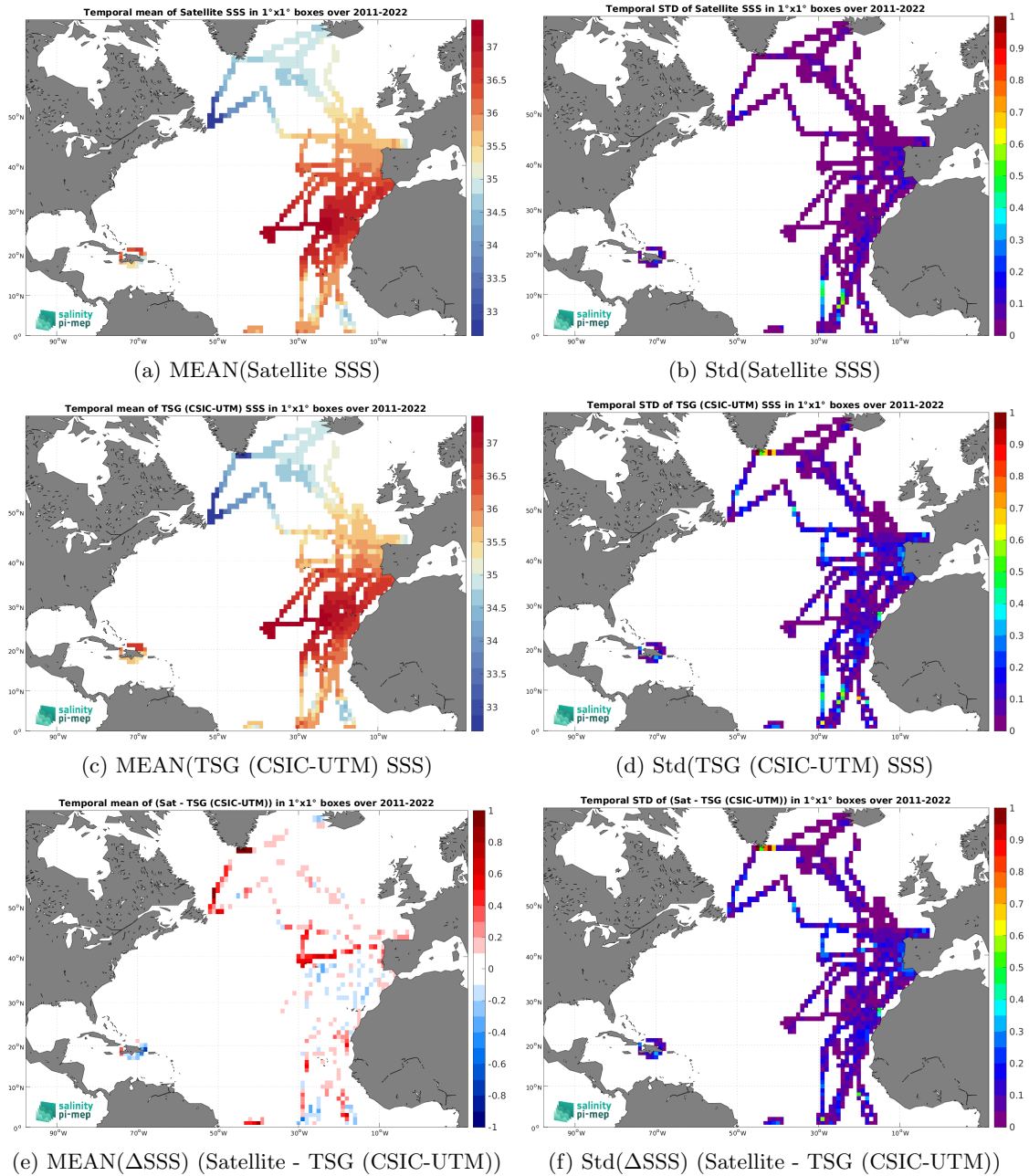
Figure 6: Temporal mean (left) and Std (right) of SSS from SMAP SSS L4 OI v2 - Monthly (IPRC) (top), TSG (CSIC-UTM) (middle), and of \Delta SSS (Satellite - TSG (CSIC-UTM)). Only match-up pairs are used to generate these maps.
