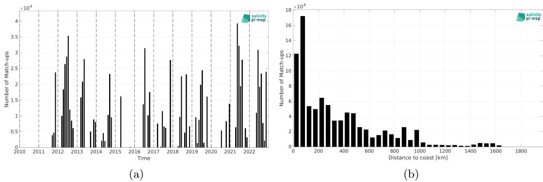
Figure 1: Number of match-ups between TSG (CSIC-UTM) and SMAP SSS L4 OI v2 - Monthly (IPRC) SSS as a function of time (a) and as function of the distance to coast (b) over the North Atlantic Ocean Pi-MEP region and for the full satellite product period.
