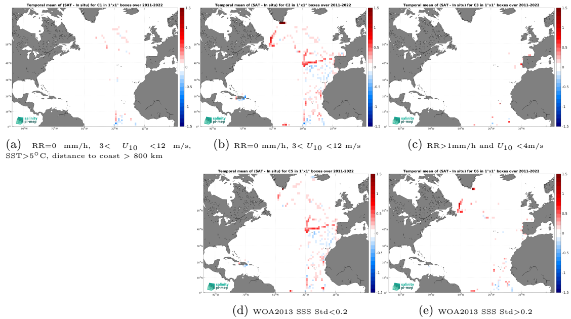
Figure 12: Temporal mean gridded over spatial boxes of size 1^\circ \times 1^\circ of \Delta\text{SSS} (SMAP SSS L4 OI v2 - Monthly (IPRC) - TSG (CSIC-UTM)) for 5 different subdatasets corresponding to:RR=0 mm/h, 3 < U_{10} < 12 m/s, SST > 5^\circ\text{C} , distance to coast > 800 km (a), RR=0 mm/h, 3 < U_{10} < 12 m/s (b), RR > 1 mm/h and U_{10} < 4 m/s (c), WOA2013 SSS Std < 0.2 (d), WOA2013 SSS Std > 0.2 (e).
