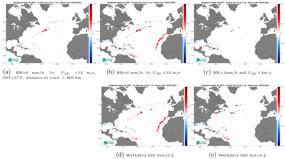
Figure 12: Temporal mean gridded over spatial boxes of size 1^\circ \times 1^\circ of \Delta\text{SSS} (SMAP SSS L4 OI v2 - Monthly (IPRC) - Saildrone) for 5 different subdatasets corresponding to:RR=0 mm/h, 3 < U_{10} < 12 m/s, SST >5^\circ\text{C} , distance to coast > 800 km (a), RR=0 mm/h, 3 < U_{10} < 12 m/s (b), RR >1 mm/h and U_{10} < 4 m/s (c), WOA2013 SSS Std <0.2 (d), WOA2013 SSS Std >0.2 (e).
