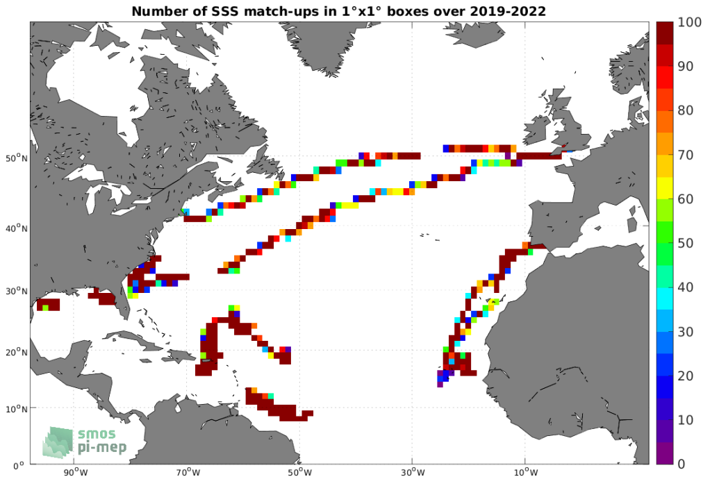
Figure 4: Number of SSS match-ups between Saildrone SSS and the SMAP SSS L4 OI v2 - Monthly (IPRC) SSS product for the North Atlantic Ocean Pi-MEP region over 1^\circ \times 1^\circ boxes and for the full satellite product period.
