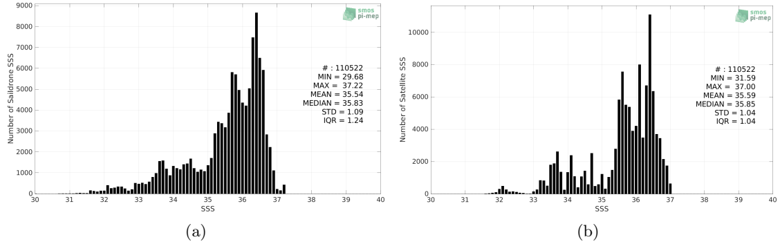
Figure 2: Histograms of SSS from Saildrone (a) and SMAP SSS L4 OI v2 - Monthly (IPRC) (b) considering all match-up pairs per bins of 0.1 over the North Atlantic Ocean Pi-MEP region and for the full satellite product period.
