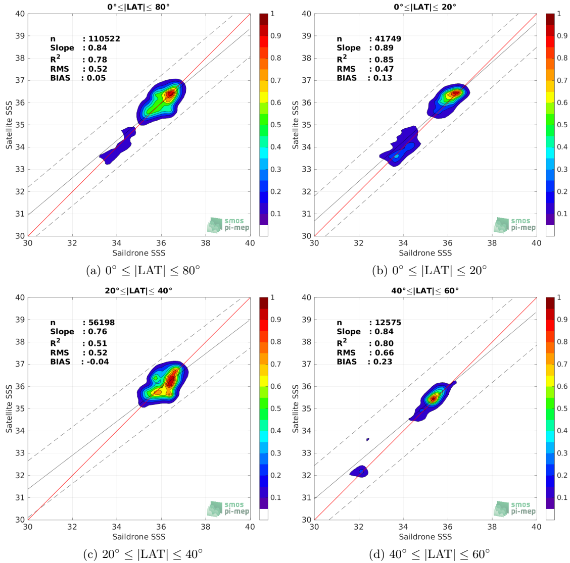
Figure 9: Contour maps of the concentration of SMAP SSS L4 OI v2 - Monthly (IPRC) SSS ( y -axis) versus Saildrone SSS ( x -axis) at match-up pairs for different latitude bands. For each plot, the red line shows x=y . The black thin and dashed lines indicate a linear fit through the data cloud and the \pm 95\% confidence levels, respectively. The number match-up pairs n , the slope and R^2 coefficient of the linear fit, the root mean square (RMS) and the mean bias between satellite and in situ data are indicated for each latitude band in each plots.
