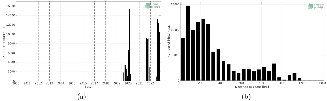
Figure 1: Number of match-ups between Saildrone and SMAP SSS L4 OI v2 - Monthly (IPRC) SSS as a function of time (a) and as function of the distance to coast (b) over the North Atlantic Ocean Pi-MEP region and for the full satellite product period.
