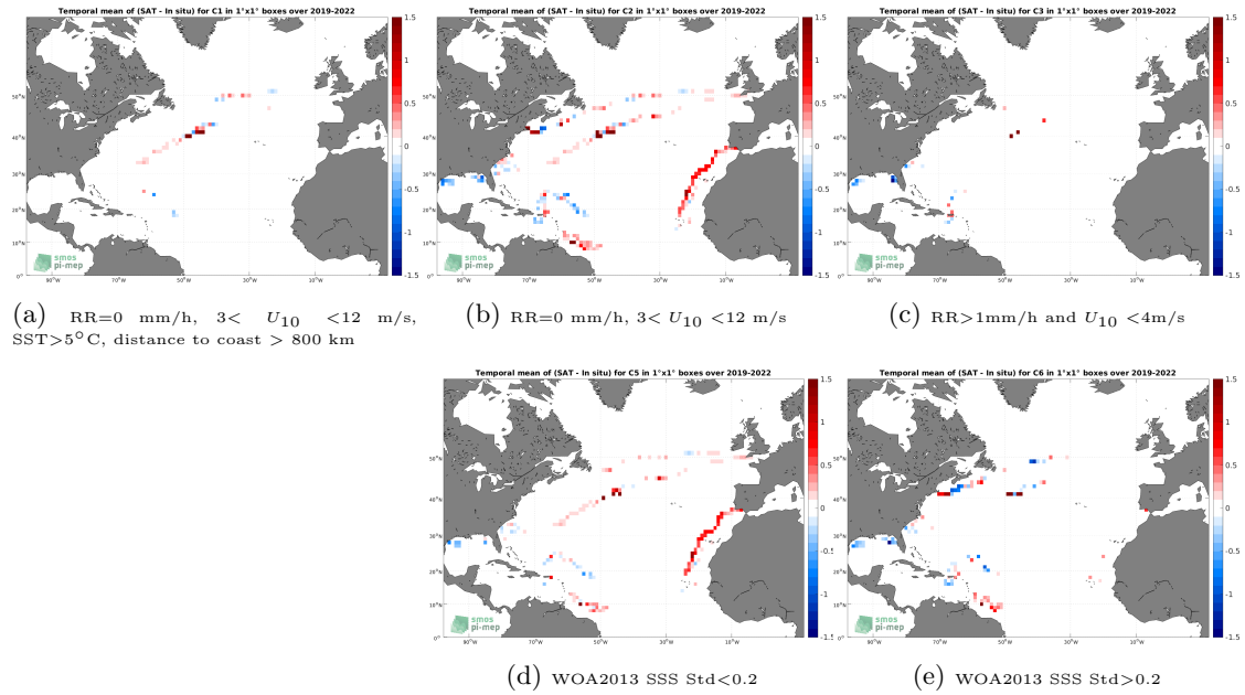
Figure 12: Temporal mean gridded over spatial boxes of size 1^\circ \times 1^\circ of \Delta SSS (SMAP SSS L4 OI v2 - Monthly (IPRC) - Saildrone) for 5 different subdatasets corresponding to:RR=0 mm/h, 3 < U_{10} < 12 m/s, SST >5^\circ\text{C} , distance to coast > 800 km (a), RR=0 mm/h, 3 < U_{10} < 12 m/s (b), RR >1 mm/h and U_{10} < 4 m/s (c), WOA2013 SSS Std <0.2 (d), WOA2013 SSS Std >0.2 (e).
