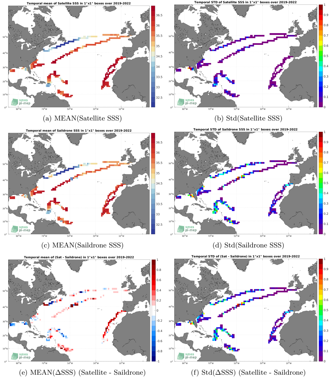
Figure 6: Temporal mean (left) and Std (right) of SSS from SMAP SSS L4 OI v2 - Monthly (IPRC) (top), Saildrone (middle), and of \Delta SSS (Satellite - Saildrone). Only match-up pairs are used to generate these maps.
