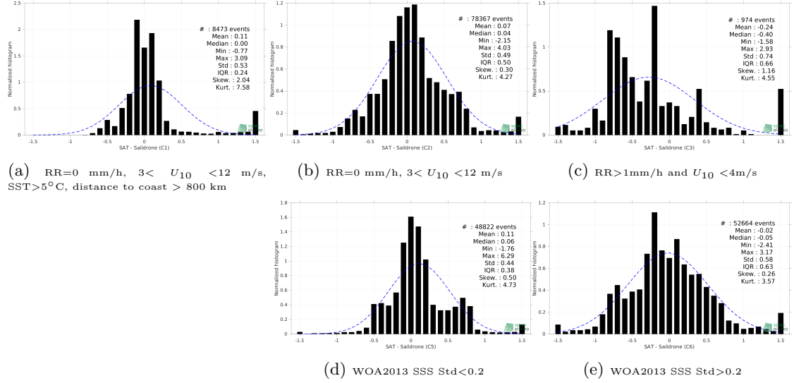
Figure 13: Normalized histogram of \Delta SSS (SMAP SSS L4 OI v2 - Monthly (IPRC) - Saildrone) for 5 different subdatasets corresponding to: RR=0 mm/h, 3 < U_{10} < 12 m/s, SST>5°C, distance to coast > 800 km (a), RR=0 mm/h, 3 < U_{10} < 12 m/s (b), RR>1mm/h and U_{10} < 4 m/s (c), WOA2013 SSS Std<0.2 (d), WOA2013 SSS Std>0.2 (e).
